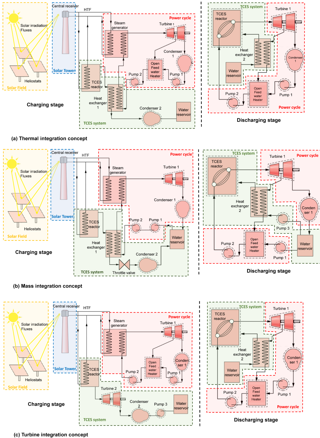
Figure 1. Schematic view of the CSP with TCES integration. (a) Thermal Int. concept; (b) Mass Int. concept; (c) Turbine Int. concept. Adapted from [26].
