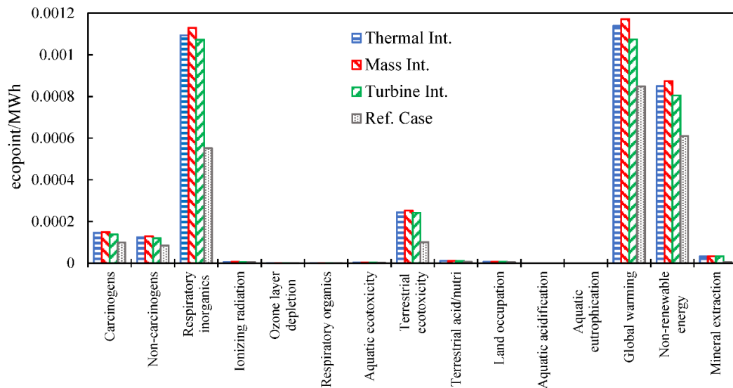
Figure 3. Comparison on normalized midpoint impacts for different TCES integration concepts.
