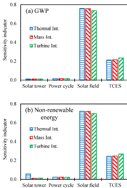
Figure 6. Sensitivity analysis results. (a) GWP; (b) Non-renewable energy
