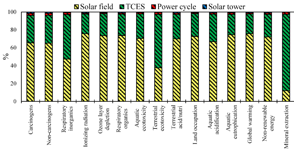
(b) Mass Int.
