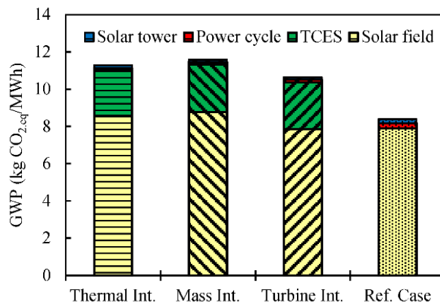
Figure 5. Global warming potential for different TCES integration concepts.
