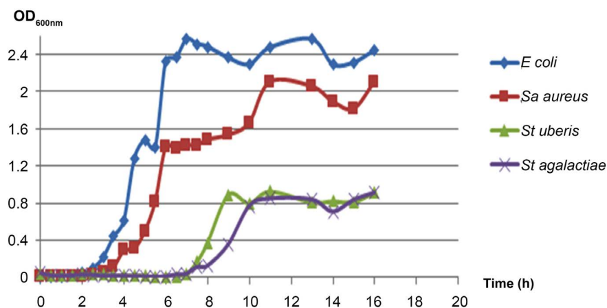
Figure 1. Growth of Escherichia coli , Staphylococcus aureus , Streptococcus uberis and Streptococcus agalactiae in BHI broth under standard conditions (pH 7.4, 37°C).
