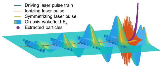
FIG. 6. The three-laser system of the resonant multipulse injection and acceleration technique [56].
