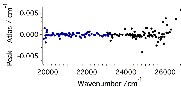
Figure 2. Scatter plot showing differences in \text{cm}^{-1} between peak positions taken from this spectrum and a selection of peak positions listed in existing atlases, mostly from ref. [2], but including peaks from ref. [5] below 19,900 \text{ cm}^{-1} and from ref. [1] above 25,000 \text{ cm}^{-1} .
