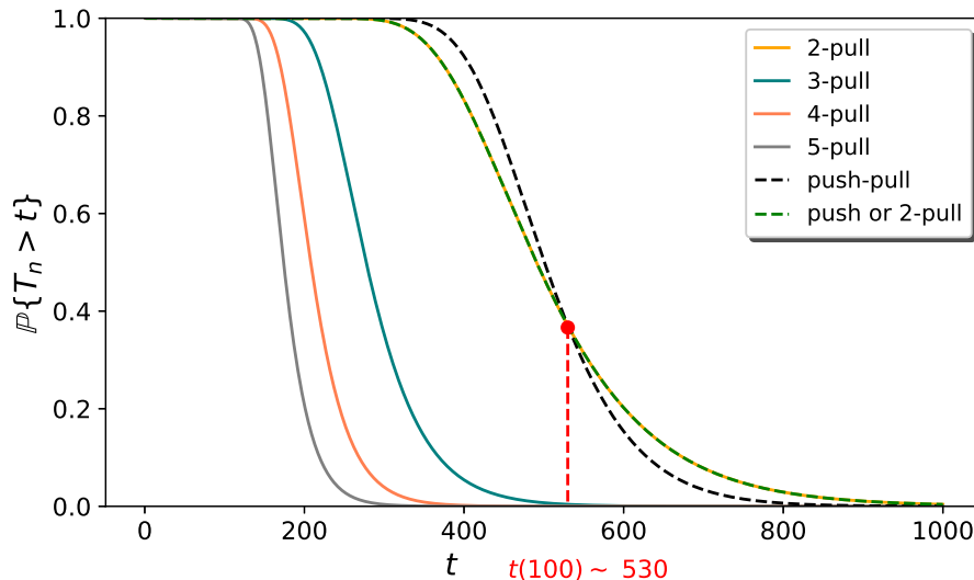
Fig. 2. Stochastic dominance illustration. Applying the algorithm detailed in Appendix B, we compute for the pull, push, push-pull and our k -pull protocols the tail probability \mathbb{P}\{T_{k,n} > t\} for n = 100 .
