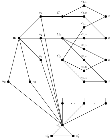
Fig. 1. First reduction from SET COVER to DISTANCE-EDGE-MONITORING SET from the proof of Theorem 19 applied to the hypergraph (\{x_1, x_2, x_3, x_4\}, \{C_1 = \{x_1, x_2\}, C_2 = \{x_2, x_3, x_4\}, C_3 = \{x_1, x_3, x_4\}\}) . Vertices and edges of V'_i and E'_i for i = 2, 3, 4 are only suggested.
