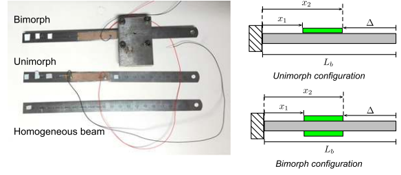
Figure 1. Photograph of the different systems under study: a homogeneous beam, a unimorph configuration, and a bimorph configuration. Sketch of the unimorph and bimorph configurations.
