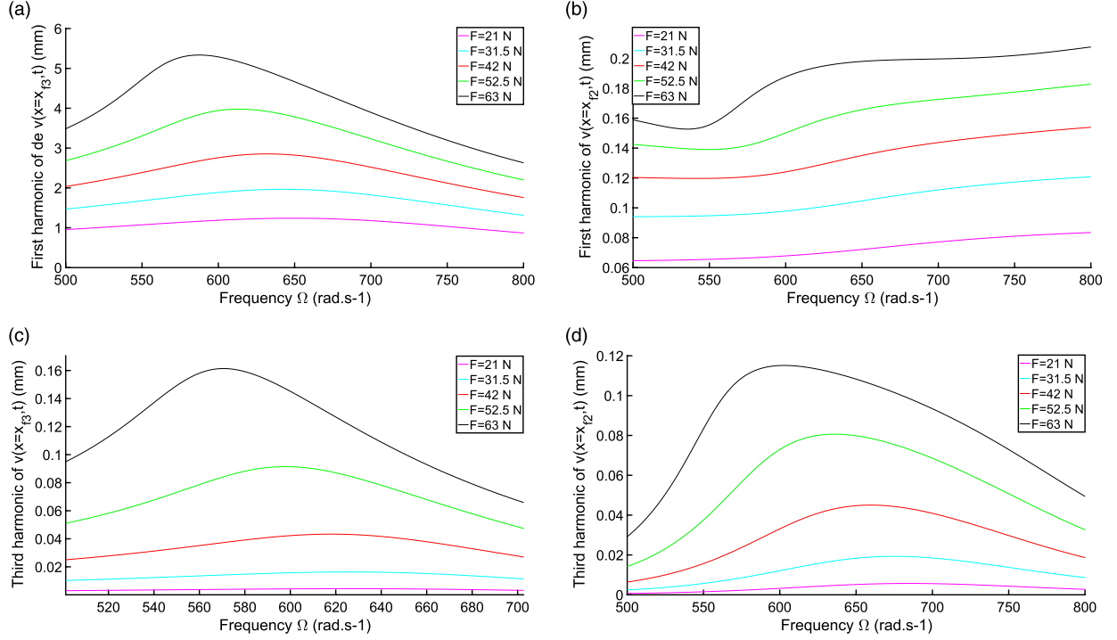
Figure 5. Theoretical results for the periodic forced response of the bimorph configuration in 1:3 internal resonance. Harmonics one and three of the displacements of the beam v(x = x_{\beta_3}, t) (low frequency—mode 2—response, left column) and v(x = x_{\beta_2}, t) (high frequency—mode 3—response, right column), as a function of the excitation frequency \Omega , for different amplitude of base acceleration (each color corresponds to a given base acceleration).
