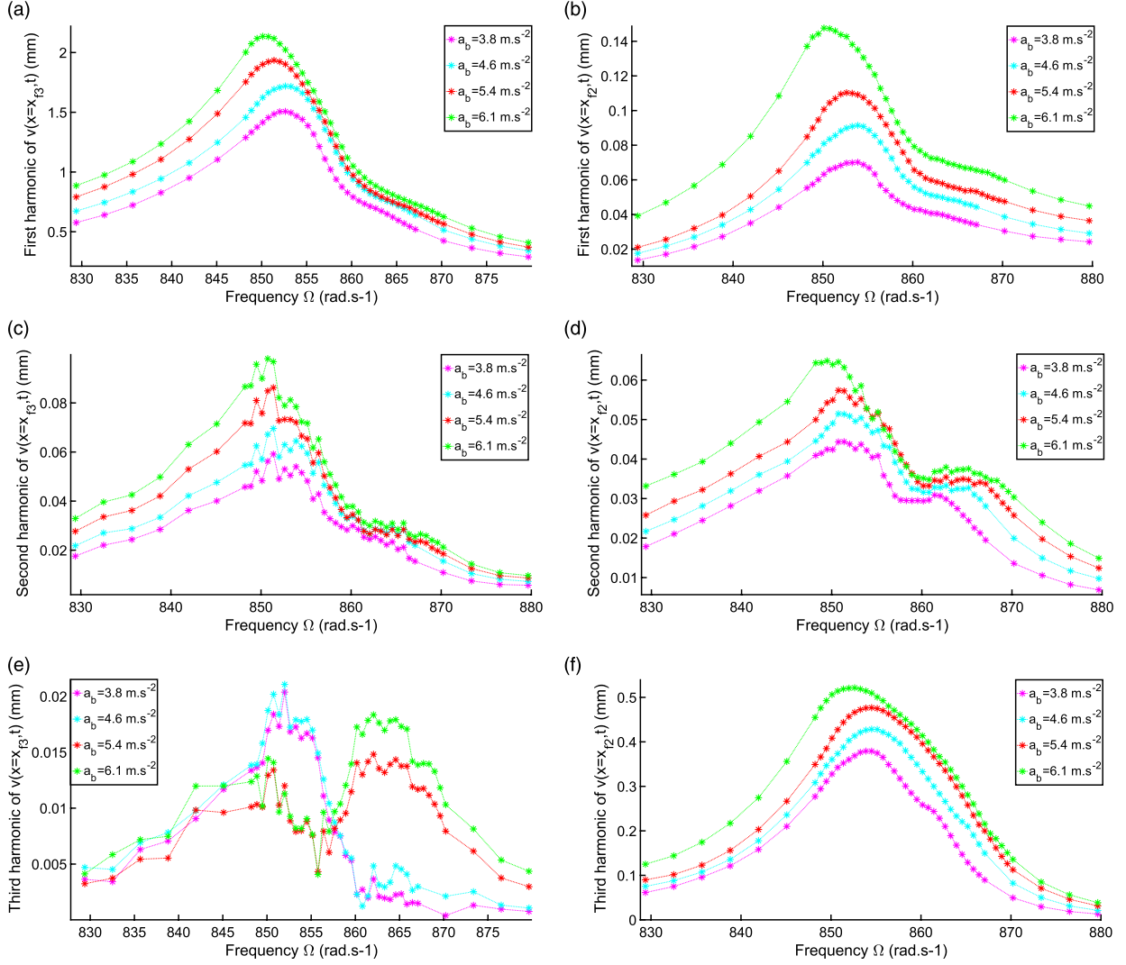
Figure 8. Experimental results for the periodic forced response of the unimorph configuration in 1:3 internal resonance. First three harmonics of the signals measured at x = x_{\beta} (low frequency—mode 2—response, left column) and x = x_{\gamma} (high frequency—mode 3—response, right column) on the beam, as a function of the excitation frequency \Omega , for different amplitude of base acceleration (each color corresponds to a given base acceleration).
