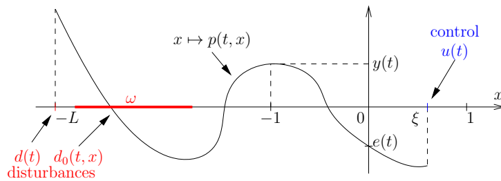
Figure 2: Illustration of the positions assumptions for the acoustic system (2).
