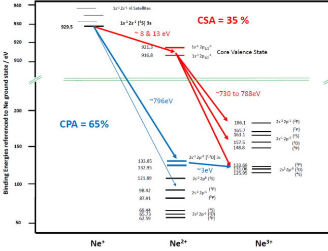
Fig. 1: (Color online) Schematic representation of CSA and CPA paths following the decay of the \text{Ne}^+ 1s2s^1 S/2p^6 3s shake up satellite. Note that for visibility the energy axis is divided into two regions, and a different y-axis scaling is used above and below the break. The corresponding paths for the 1s2s^1 S/2p^6 3s state are similar (except that 1 st step CSA and CPA Auger electrons have then respectively 14/19eV and 802eV). Energy levels are from NIST tables, except for the levels in red and blue which are obtained from our experiment.
