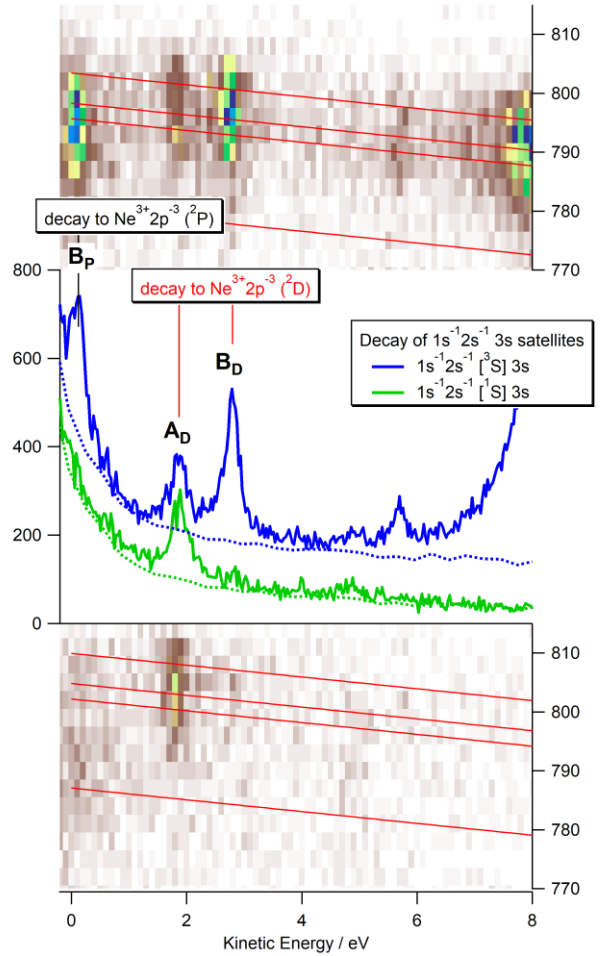
Fig. 7 Center: Spectra of the low energy electrons emitted upon Auger decay of the \text{Ne}^+ 1s2s^3S^2p^63s state. The dotted lines indicate an estimate of the background of false coincidences, obtained from coincidences with electrons in the red zone of Fig 3 B). A vertical offset of 100 is used for the upper curves to separate them from the lower ones. Top and bottom show the energy correlation map between the slow (x-axis) and the fast (y-axis) Auger electrons detected in coincidence with the \text{Ne}^+ 1s2s^3S^2p^63s photoelectron (top) or with the one \text{Ne}^+ 1s2s^3S^2p^63s photoelectron (bottom).
