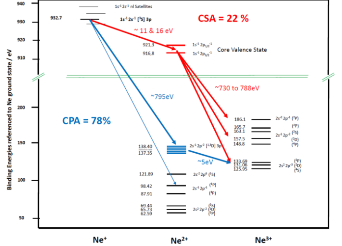
Fig. 2: (Color online) Schematic representation of CSA and CPA paths following the decay of the \text{Ne}^+ conjugate shake up satellite 1s2s^1 S/2p^6 3p . It is similar to Figure 1 which describes the decay of the \text{Ne}^+ normal shake up satellite. The corresponding paths for the 1s2s^1 S/2p^6 3p state are similar (except that 1 st step CSA and CPA Auger electrons have then respectively 17/22 and 801eV).
