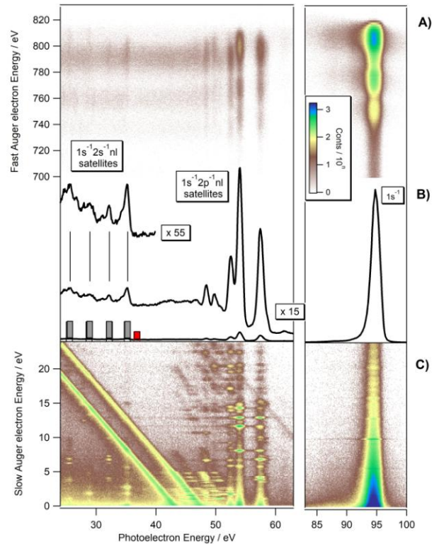
Fig. 3: (Color on line) Fast and slow Auger decays of Ne 1 s satellites. B) is the photoelectron spectrum. The two-dimensional (e,e) coincidence maps, reveal the detection of the fast (A) and slow (C) Auger electron in coincidence with their associated photoelectron. The gray and red zones highlighted in (B) show the energy ranges used for the true and false coincidence spectra in Fig. 4
