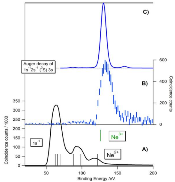
Fig 5 \text{Ne}^{2+} states populated by the Auger decay of \text{Ne}^+ 1s^{-1} state (A) or by CPA decay of the \text{Ne}^+ 1s2s[{}^3S]2p^63s state (B is experiment, C, our calculation). Experimental curves are obtained from the Auger spectra observed in coincidence with the corresponding photoelectrons, in the energy range defined in Fig. 3 B) by the grey rectangles. Conversion of the E_A \sim 800\text{eV} fast Auger electron energies into binding energy B_{En} of the \text{Ne}^{2+} states populated by the Auger decay is given by B_{En} = B_{E^+} - E_A where B_{E^+} is the binding energy of the initial hole-state. Vertical lines indicate \text{Ne}^{2+} levels and \text{Ne}^{3+} threshold from the NIST data base. Note that for (B) false coincidences have been subtracted; they are estimated from coincidences with electrons in the red zone in Fig 3 B) and contain also an estimate of the pollution by the core valence direct DPI path (2). The resulting spectrum in (B) includes a weak contribution of the fast Auger electrons emitted in the 2 nd step CSA decay; however their lower kinetic energies than the 1 st step CPA electrons converts into a contribution and an asymmetry on the high binding energy side of the experimental peak.
