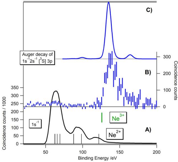
Fig. 6: (Color online) Equivalent of Fig 5 but for the \text{Ne}^+ conjugate shake up satellite 1s2s^3S^2p^63p . As for Fig. 5, the experimental CPA Auger spectrum in B) is obtained from the spectrum of electrons detected in coincidence with the 1s2s^3S^2p^63p photoelectron line, selected in the grey zone of Fig. 3 B). False coincidence and an estimate of the pollution by the direct Core Valence Double ionization to \text{Ne}^{2+} 1s2s^2p^5 (^1,^3P) states are subtracted. These contributions were estimated from the spectrum of electrons detected in coincidence with electrons selected in the red zone of Fig. 3 B)
