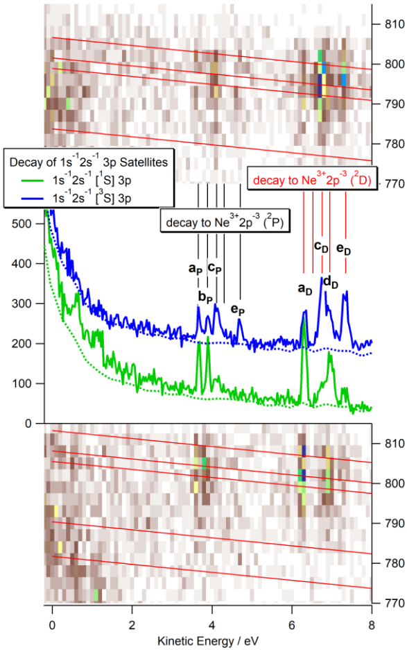
Fig. 8 Center: Spectra of the low energy electrons emitted upon Auger decay of the \text{Ne}^+ 1s2s[{}^1\text{S}]2p^63p state. Similar to Fig. 7, the top and bottom maps show the energy correlation maps between the slow (x-axis) and the fast (y-axis) Auger electrons detected in coincidence with the \text{Ne}^+ 1s2s[{}^3\text{S}]2p^63p photoelectron (top) or with the one \text{Ne}^+ 1s2s[{}^1\text{S}]2p^63p photoelectron (bottom).
