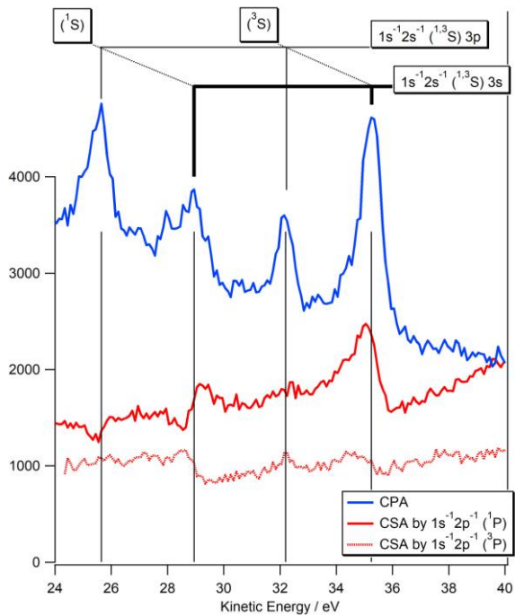
Fig. 4: (Color on line) Comparison of the relative probabilities of the CPA and CSA paths, deduced from Fig. 2. The CSA paths through the \text{Ne}^{2+} 1s2s2p^5 (^3P) and (^1P) paths are differentiated. See text for details.
