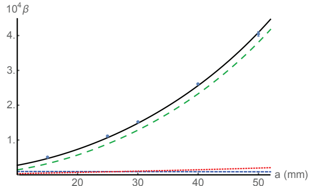
Fig. 3 The experimental and theoretical values of \beta = -F'_x/v_x in kg/s are plotted as a function of the sphere radius a . The blue dots represent the experimental values \beta_{exp} , with their error bars. The curves represent the theoretical value of \beta_{S1} (red dotted curve), \beta_{S2} (long dashed green curve), \beta_W (short dashed blue curve) and their sum \beta_{th} (full line black curve). The quantities \beta_{S1} and \beta_{S2} include the correction by confinement calculated for a sphere of radius b = 140 mm, chosen as it gives the best fit to the measurements. The theoretical functions take into account the variation of the viscous penetration depth \delta with the sphere radius a because the pendulum frequency is a function of a , namely \omega/(2\pi) mHz = 878 - 2.42a with a in mm.
