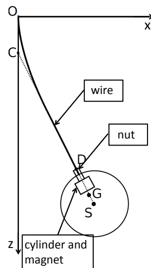
Fig. 1 Schematic drawing of the pendulum. The suspension wire is fixed in O in the support and in D in the pendulum body. G is the center of mass of the body and S is the center of the sphere. C is the center of rotation of the pendulum body and C would coincide with O if the wire rigidity was negligible. The oscillation amplitude x_0 has been grossly exaggerated with respect to the experimental values x_0 \leq 0.6 mm while the wire length OD is l_W = 404 \pm 0.5 mm.
