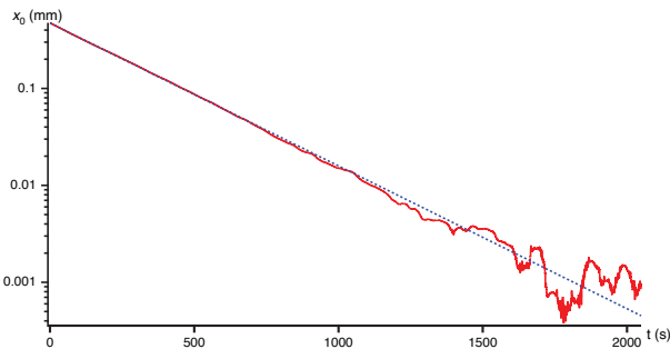
Fig. 2 The amplitude x_0(t) (mm) is plotted as a function of the time t (s): measured values (full red line) and their best fit (dotted blue line). The semi-logarithmic plot proves that the agreement of the fit extends until the x_2 term is no more negligible.
