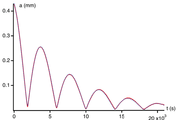
Fig. 4 Damping of the oscillation of the sphere of radius a = 15 mm under vacuum. The measured amplitude x_0(t) is plotted as a function of the time t (s) (full red line) and its fit using eq. (28) (dashed blue line). The damping time constant \tau and the beat period T_0 given by the fit are \tau = 7174 s and T_0 = 4061 . The amplitudes A and B mm are almost equal in this experiment: this condition, which maximizes the beat contrast, occurs if \theta \approx \pm\pi/4 .
