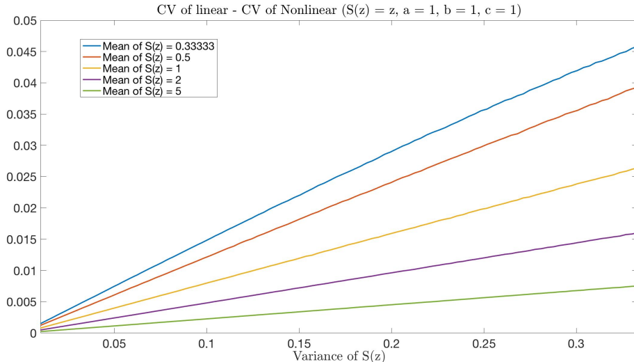
Figure 1: CV_L - CV_{NL} as a function of the variance of S(z) for different values of the mean of S(z) when a = b = c = 1 , S(z) = kz + d , for k \in [0, 2] and d = 1/3, 1/2, 1, 2, 5 , where z follows the uniform distribution in [-1/2, 1/2] .
