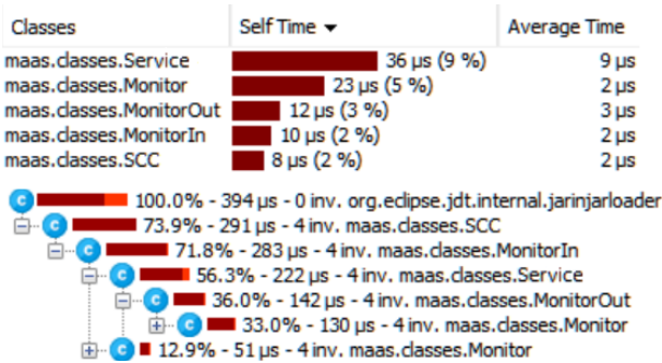
Fig. 14 CPU allocation.
