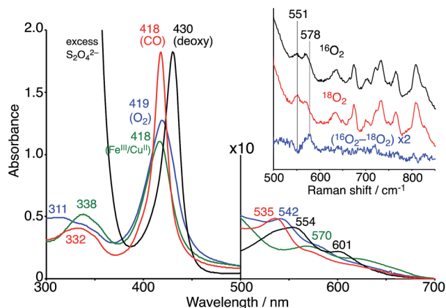
Fig. 5 UV-vis spectra of the Fe III TPPS/Cu I TerpyCD 2 (green) and its reduced Fe II TPPS/Cu I TerpyCD 2 complexes in the deoxy (black), oxy (blue) and CO (red) forms in 0.05 M phosphate buffer at pH 7.0 and 25 °C. The inset shows the resonance Raman spectra of the Fe II TPPS/Cu I TerpyCD 2 complexes obtained by excitation at 405 nm under 16 O 2 atmosphere (black), 18 O 2 atmosphere (red), and the difference 16 O 2 - 18 O 2 (blue). Conditions: 0.05 M phosphate buffer at pH 7.0, 77 K (frozen solution).
