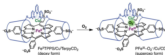
Fig. 6 Oxygenation of the Fe II TPPS/Cu I TerpyCD 2 complex to form a superoxo PFe III -O 2 - /Cu I CD 2 complex.
