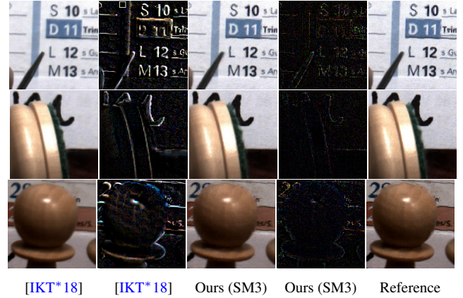
Figure 9: Visual comparison of our method using SM3 versus Inagaki et al. [IKT*18] for three data sets: Boxer-Gladiaator-Irish , Chess , and Chess-moving ; shown from top to bottom, respectively. For quantitative results see tables 2 and 3. Error insets have a 5x intensity scaling to facilitate comparisons.
