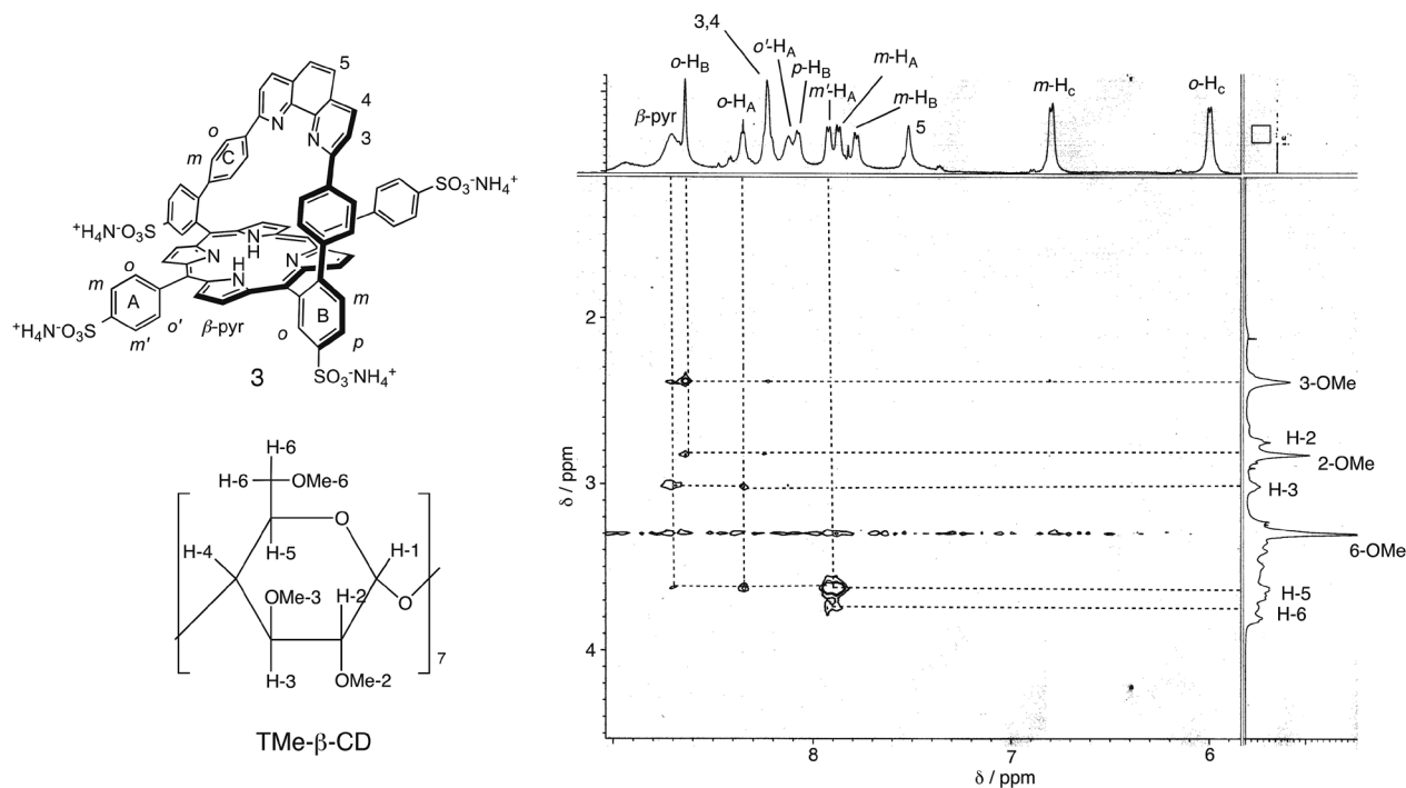
Fig. 2. ROESY NMR spectrum of the 2:1 TMe- \beta -CD/ 3 complex ( [\text{TMe-}\beta\text{-CD}] = 2 \text{ mM} , [\mathbf{3}] = 1 \text{ mM} ) in \text{D}_2\text{O} at 25^\circ\text{C} . The mixing time was 0.25 s
