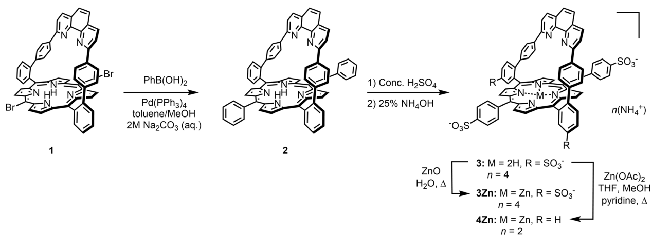
Scheme 1. Synthesis of sulfonated zinc porphyrins
