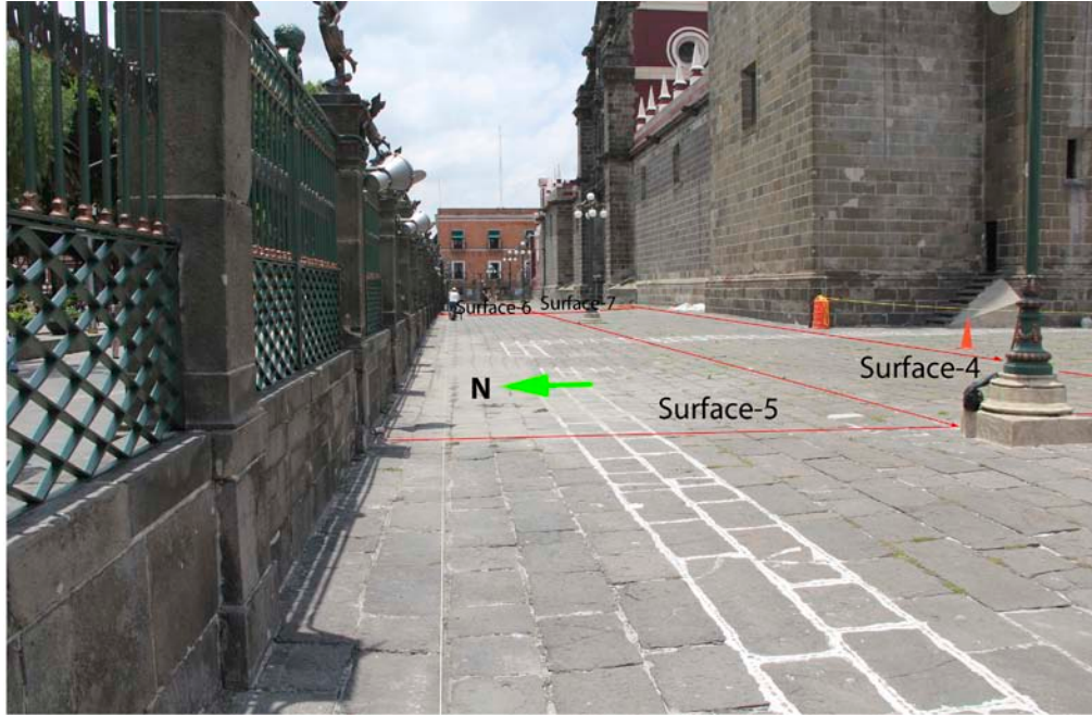
Fig. 4. North side of the cathedral, note the distribution of the four surfaces prospected with a 400 MHz GPR antenna (S4, S5, S6 and S7 areas).
