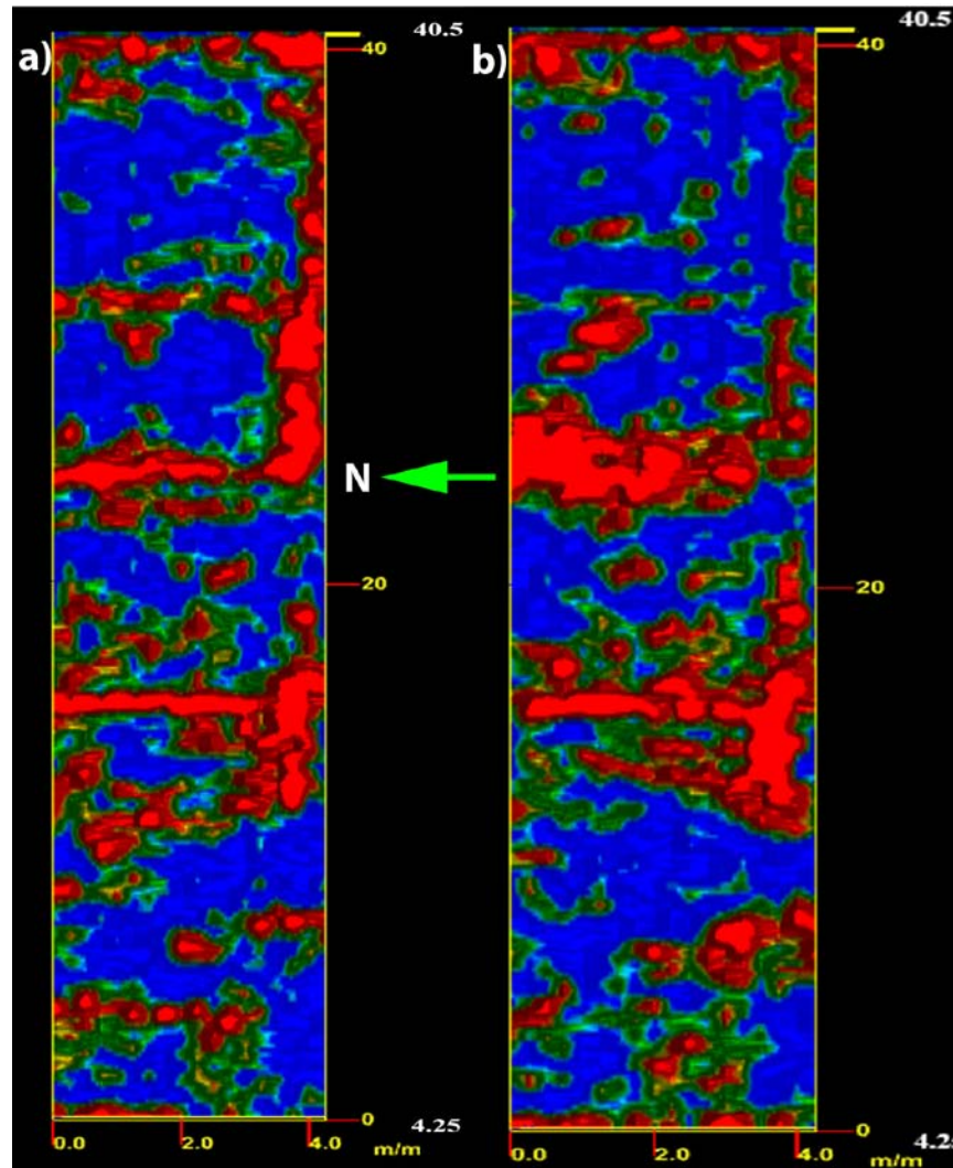
Fig. 11. Depth slices at 1 m (a) and 1.5 m (b) depth in the S6 area. The red anomalies show high reflectivity zones, probably corresponding to remains of buried construction structures.
