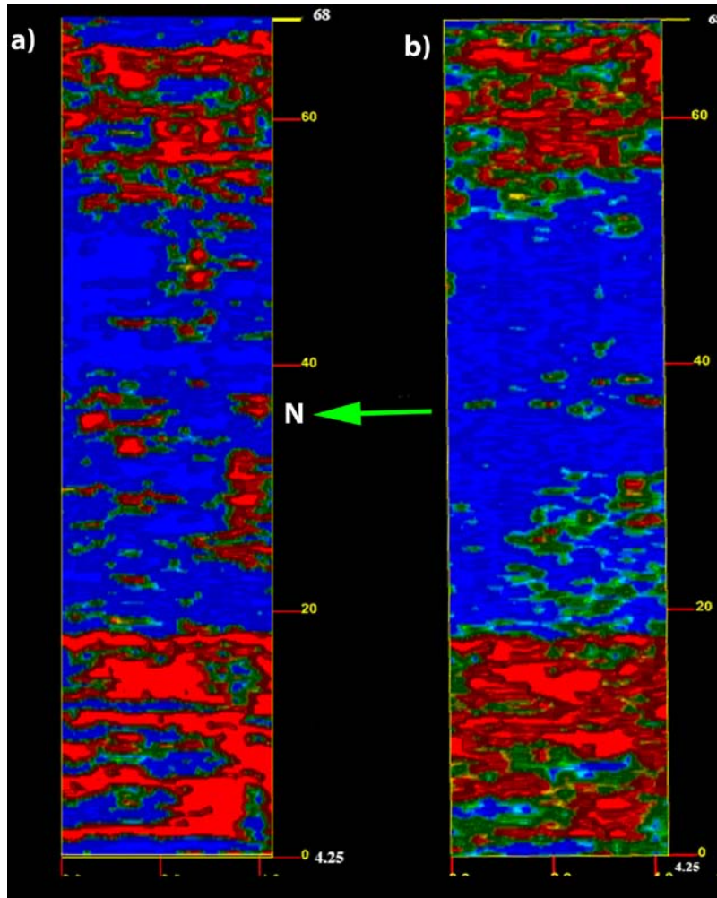
Fig. 10. Depth slices at 1 m (a) and 1.5 m (b) depth in the S5 area. The red anomalies indicate highly reflective zones and probably correspond to old foundations.
