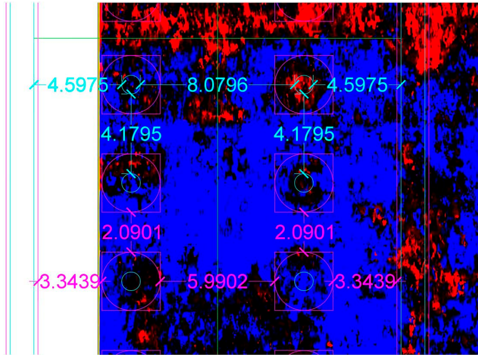
Fig. 14. The numbers show the distances from the columns to the walls, between the columns and between both rows of columns: a) in blue the centre to centre distance; b) in magenta from the bases of the columns.
