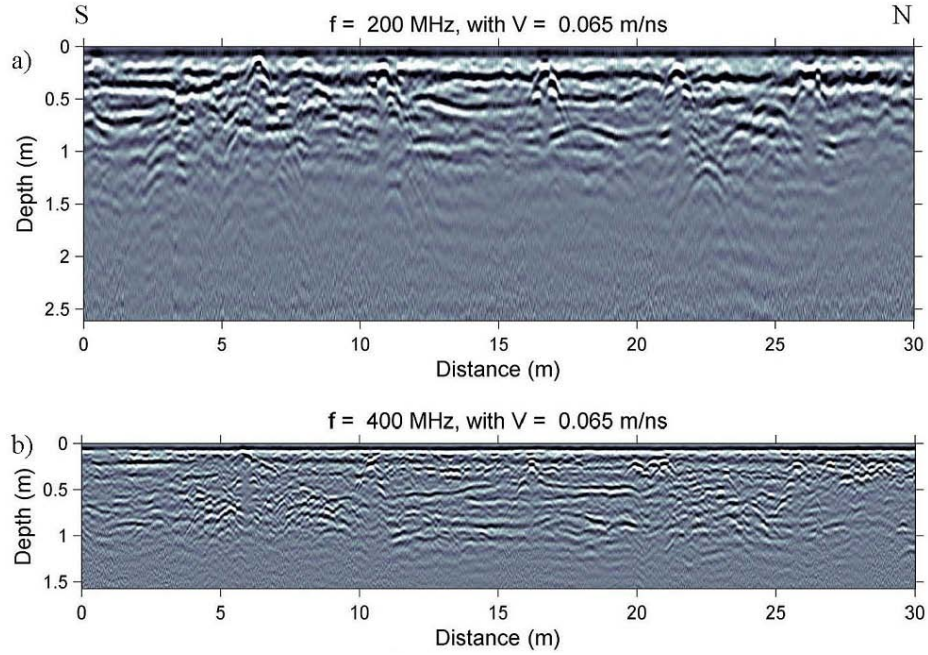
Fig. 5. Example of a 2D GPR profile measured on the Surface-1 with a) 200 and b) 400 MHz antennas, respectively. We only show the first thirty meters of profile1. Note the presence of multiple reflections/diffractions coming from archeological buried structures.
