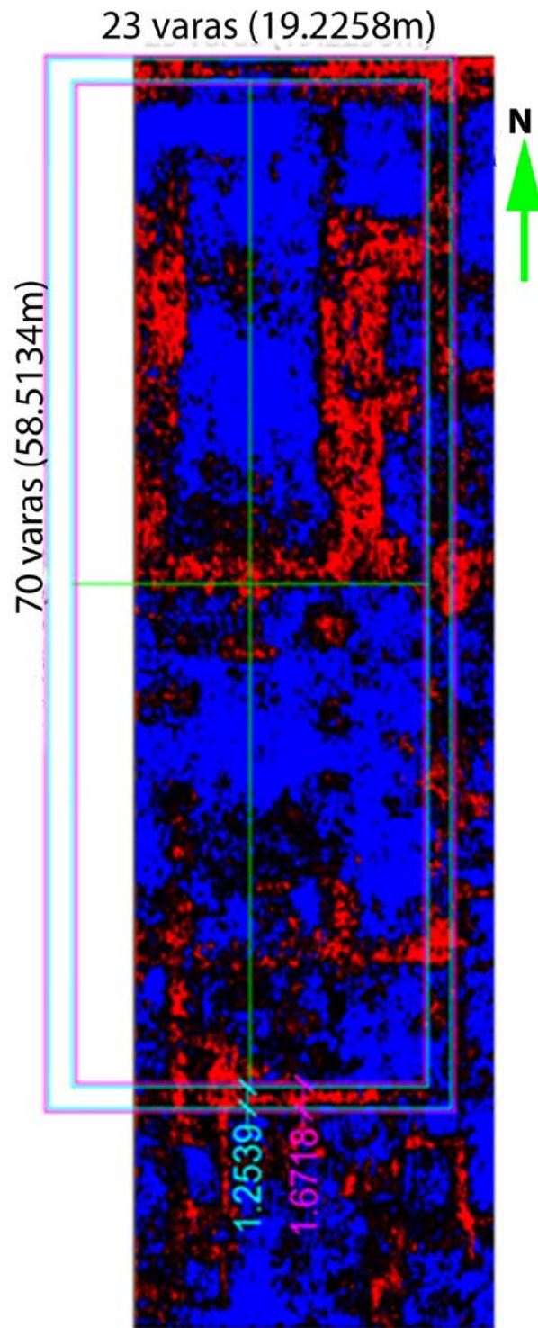
Fig. 13. Depth slice of S1 area at 1 m depth. Note the presence of ‘El Sagrario’ in the northern part (see the blue zone cross-shaped area). The light blue rectangle demarcates the area of the ancient temple where the thickness of the walls is estimated to be about 1.2539 m, and the magenta color refers to the foundations about 1.6718 m thick.
