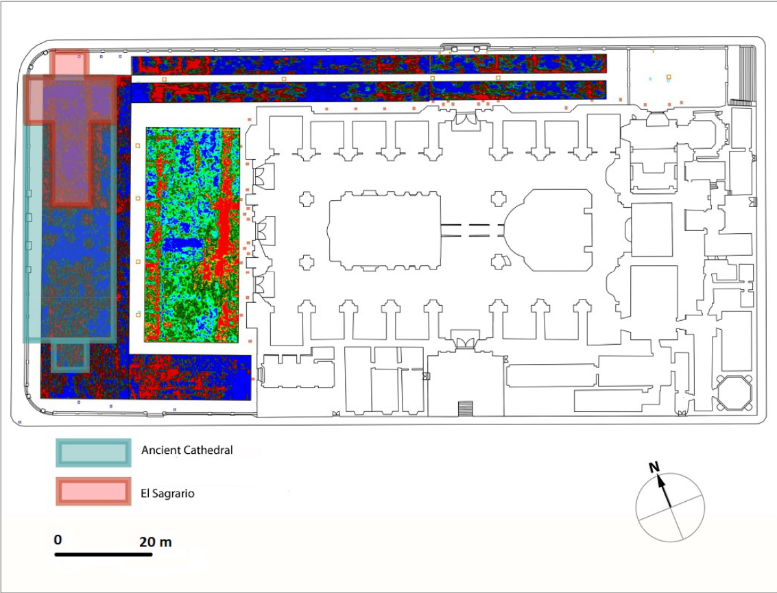
Figure 17 Architectural plans with the integration of all GPR results.
