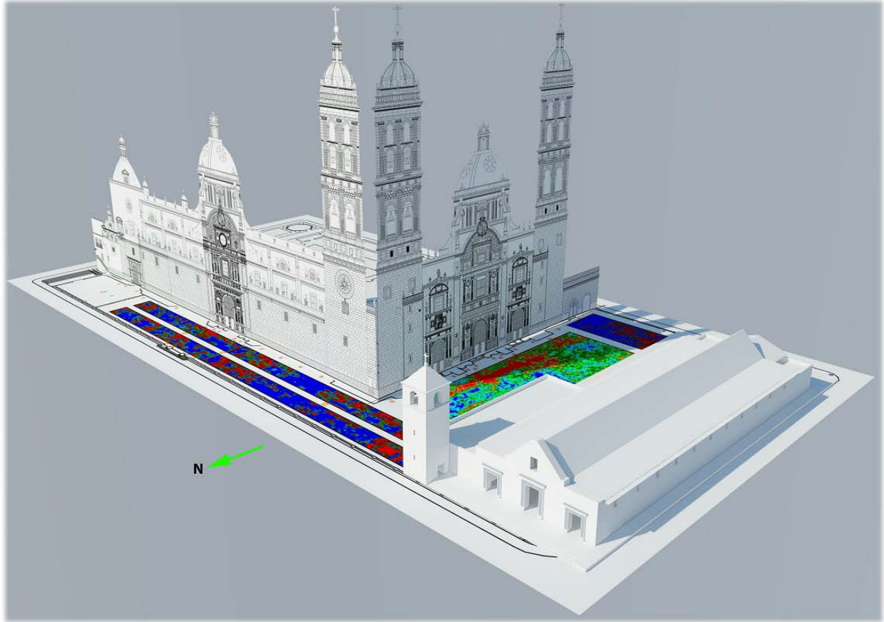
Fig. 18. 3D model integrating the ancient temple at the front with the current cathedral in the background and the depth slices of GPR images at 1 m depth showing the remains of building foundations interpreted as chapels.
