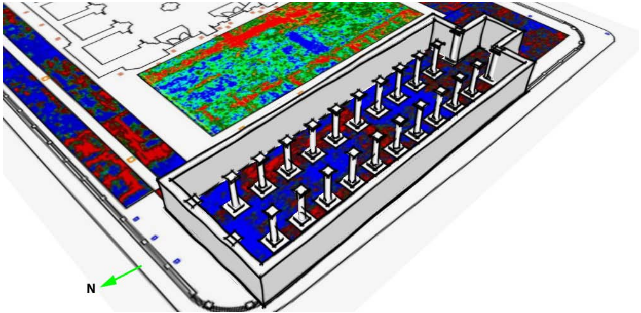
Fig. 15. Hypothetical reconstructions of the columns from the GPR depth slice in background. The red anomalies indicate the reflective zones corresponding to walls and construction structures.
