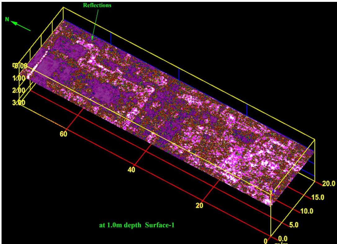
Fig. 6. 3D presentation of S1 area at a depth of 1 m (depth slice); the antenna used is of 400 MHz.
