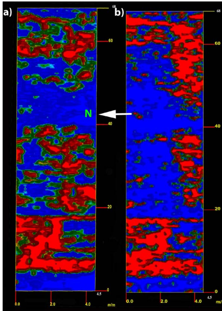
Fig. 9. S4 area in the northern part of the cathedral. Depth slices at 1m(a) and 1.5 m (b) depth, respectively. The red anomalies show zones with high reflectivity and could correspond to old foundations.
