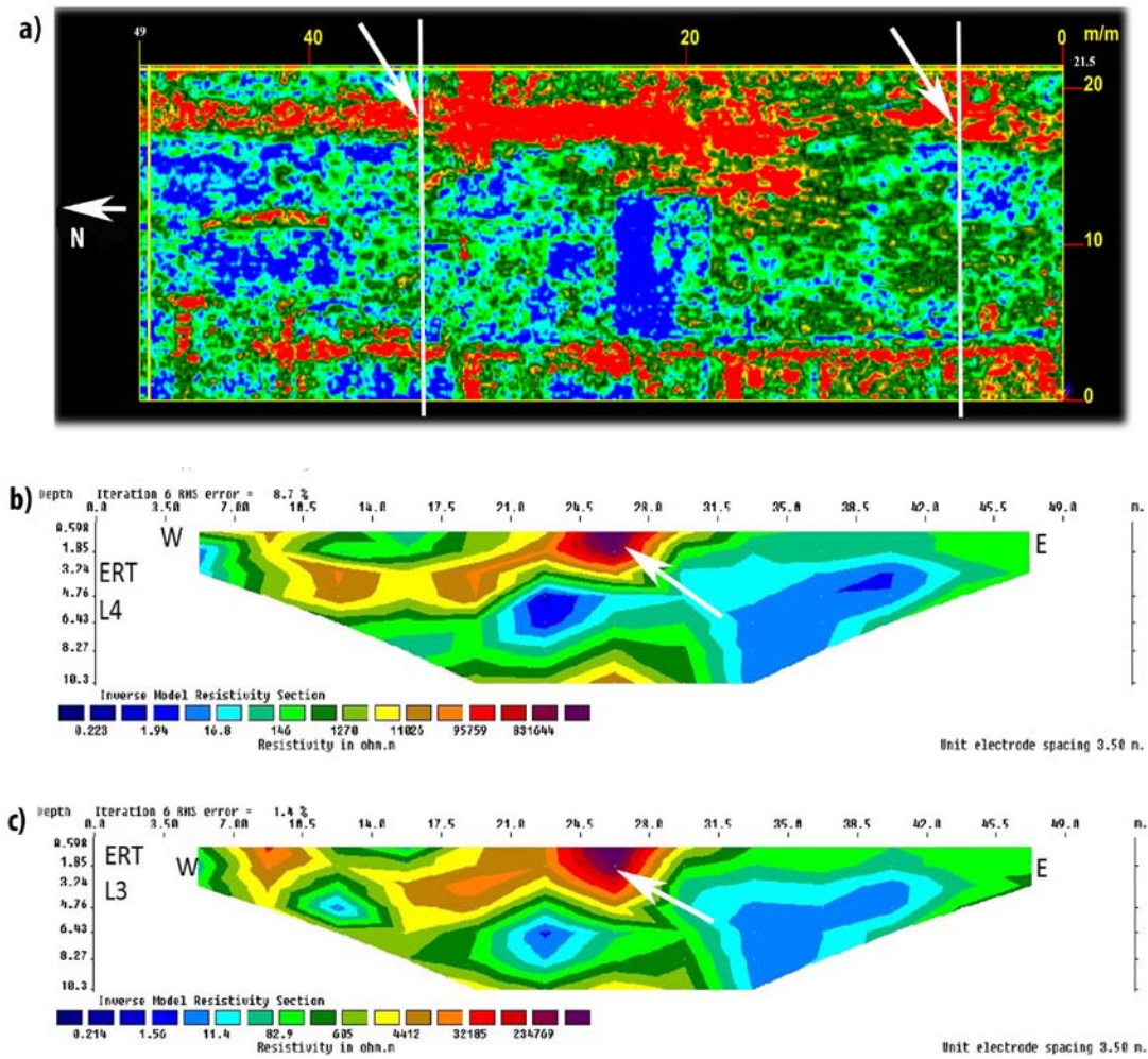
Fig. 7. a) The depth slice at 1 m depth with a 400 MHz antenna, S2 area. Note the distribution of the reflections (in red) coming probably from a well-defined geometric settlement. b) and c) show the ERT profiles L-4 (white line on the left) and L-3 (white line on the right), respectively. The white arrows indicate high resistive anomalies in accordance with high reflective zones (in red) shown by white arrows in the depth slice of a)
