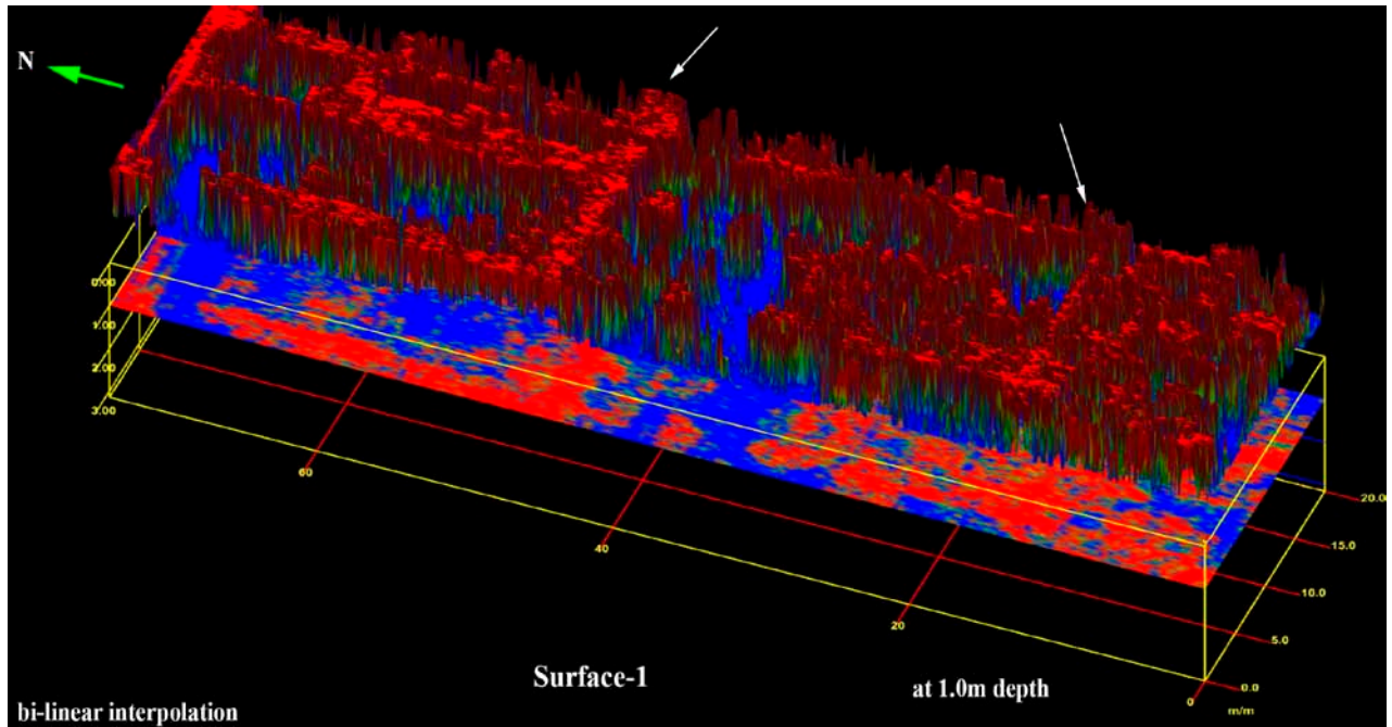
Fig. 12. Depth slice of S1 area at 1 m depth presented in 3D using cross and in-lines interpolation of the data (bilinear interpolation). The most reflective areas in red, indicated by white arrows, define buried geometric building structures.
