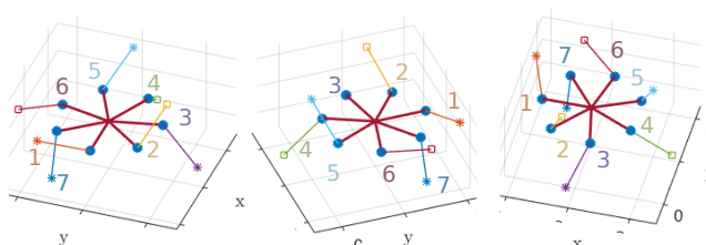
Fig. 2: Optimized propeller direction of the O_+^7 design, with n = 7 , d = 0.16 [m] and k = 0.002 [m] at \text{cond}(\Sigma^{-1} \mathbf{F}) = 2.052 .
