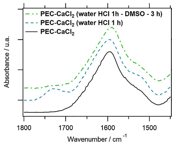
Fig. 3. FTIR spectroscopy of PEC- \text{CaCl}_2 , PEC- \text{CaCl}_2 treated with HCl in water (1 h) and followed by an acid-free DMSO bath (3 h).
