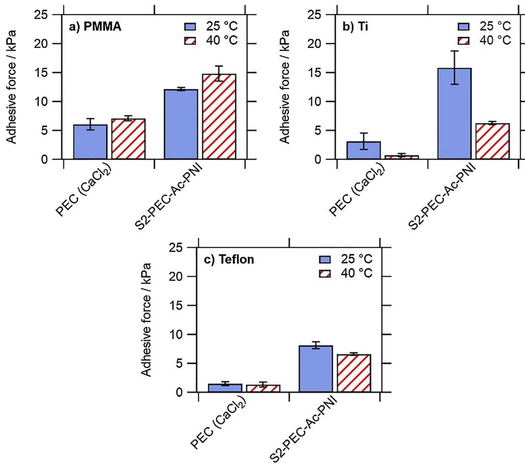
Fig. 8. Adhesive forces between the model surfaces and the PECs, at 25 °C and 40 °C, with or without surface modifications.
