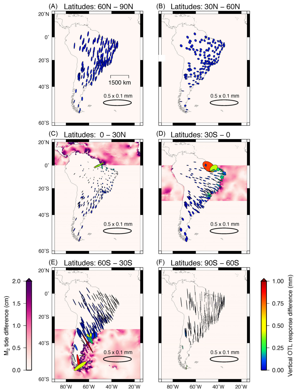
Figure 18. Predicted M_2 OTL-induced surface displacements across South America due to the direct differences between the ocean-tide models FES2012 and TPX08-Atlas, partitioned into six latitudinal bands: (a) 60^\circ\text{--}90^\circ\text{N} , (b) 30^\circ\text{--}60^\circ\text{N} , (c) 0^\circ\text{--}30^\circ\text{N} , (d) 30^\circ\text{--}0^\circ\text{S} , (e) 60^\circ\text{--}30^\circ\text{S} and (f) 90^\circ\text{--}60^\circ\text{S} . Note that the PME in panel (f), derived from ocean-tide model discrepancies around the Antarctic continent, are oriented strongly in the north–south direction and exhibit non-diminishing amplitudes as a function of distance from the coast ( cf. Fig. 3). The colour bar to the left of panel (e) represents the magnitude of the vector differences between ocean-tide models and the colour bar to the right of panel (f) represents the predicted OTL-induced vertical displacement due to the ocean-tide differences.
