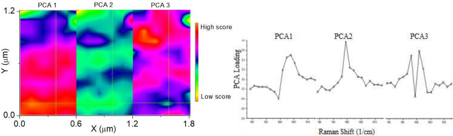
Figure 7- Results of PCA scores obtained from x,y profiles and one-dimensional PCA-loadings plot performed on the 900\text{-}1015\text{ cm}^{-1} spectral map of TMJ disc samples before and after M.S.
