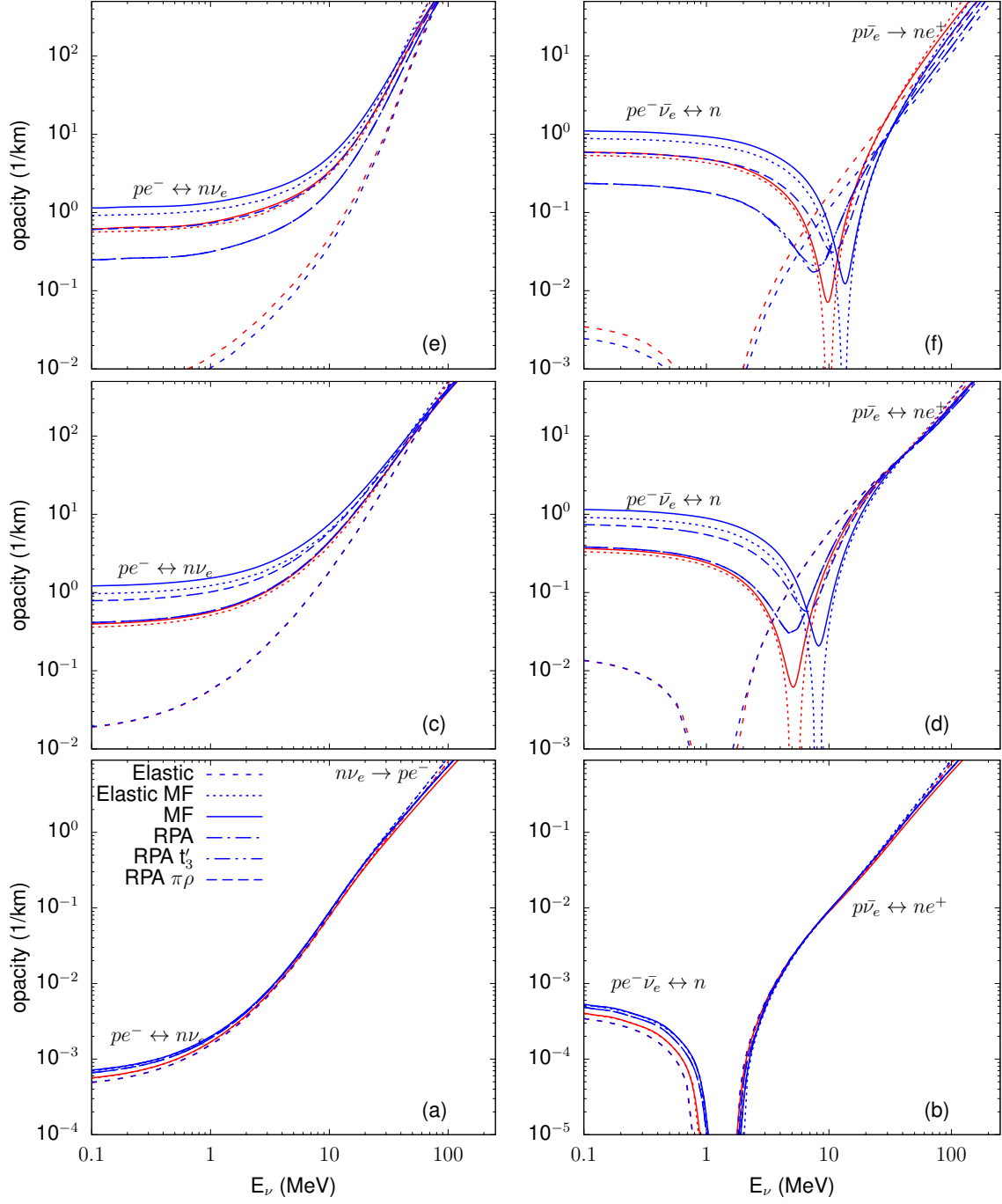
FIG. 3: (color online) Neutrino (left) and anti-neutrino (right) opacities for T = 12 MeV, n_B = 0.01 \text{ fm}^{-3} and Y_e = 0.1 (upper panels), T = 19 MeV, n_B = 5 \times 10^{-3} \text{ fm}^{-3} and Y_e = 0.1 (middle panels) and T = 5 MeV, n_B = 10^{-4} \text{ fm}^{-3} and Y_e = 0.1 (lower panels). These correspond to typical conditions close to the neutrinosphere in a CCSN from our fiducial simulation, see section III. The different line types distinguish the different approximations and results with HS(DD2) are indicated in red, whereas those with RG(SLy4) are in blue. The dominant processes contributing to the opacities in a certain energy domain are mentioned in the figure, too.
