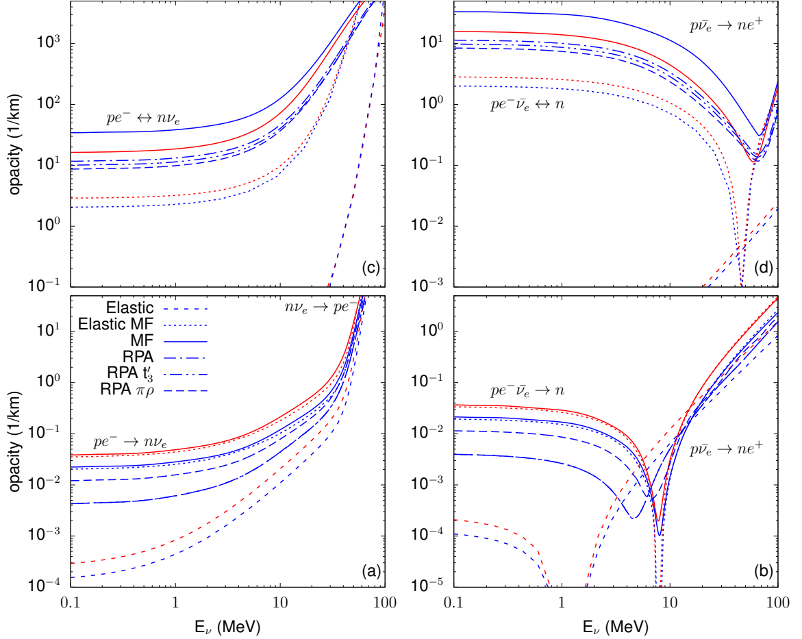
FIG. 2: (color online) Neutrino (left) and anti-neutrino (right) opacities for T = 8 MeV, n_B = 0.11 \text{ fm}^{-3} and Y_e = 0.05 (upper panels), and T = 5 MeV, n_B = 0.01 \text{ fm}^{-3} and Y_e = 0.15 (lower panels). These correspond to typical conditions for the decoupling of neutrinos in the merger remnant [59], the former are more relevant for lower neutrino energies than the latter. The different line types distinguish the different approximations and results with HS(DD2) are indicated in red, whereas those with RG(SLy4) are in blue, see section II B for details. The dominant processes contributing to the opacities in a certain energy domain are mentioned in the figure, too.
