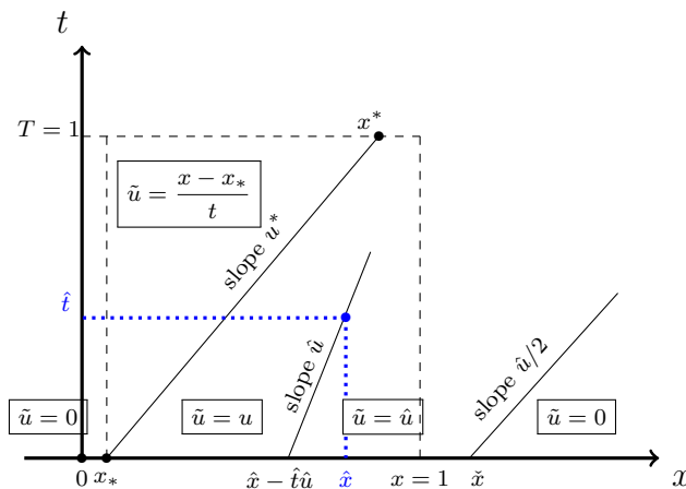
Figure 4: Modification of the auxiliary function \tilde{u} (cf. Fig. 1): construction based upon the existence of a point (\hat{x}, \hat{t}) \in (0, 1) \times (0, 1) with \hat{x} > x^* - (1 - \hat{t})u^* such that \hat{u} := u(\hat{x}, \hat{t}) > 0 ; the point \hat{x} > \hat{x} is arbitrary.
