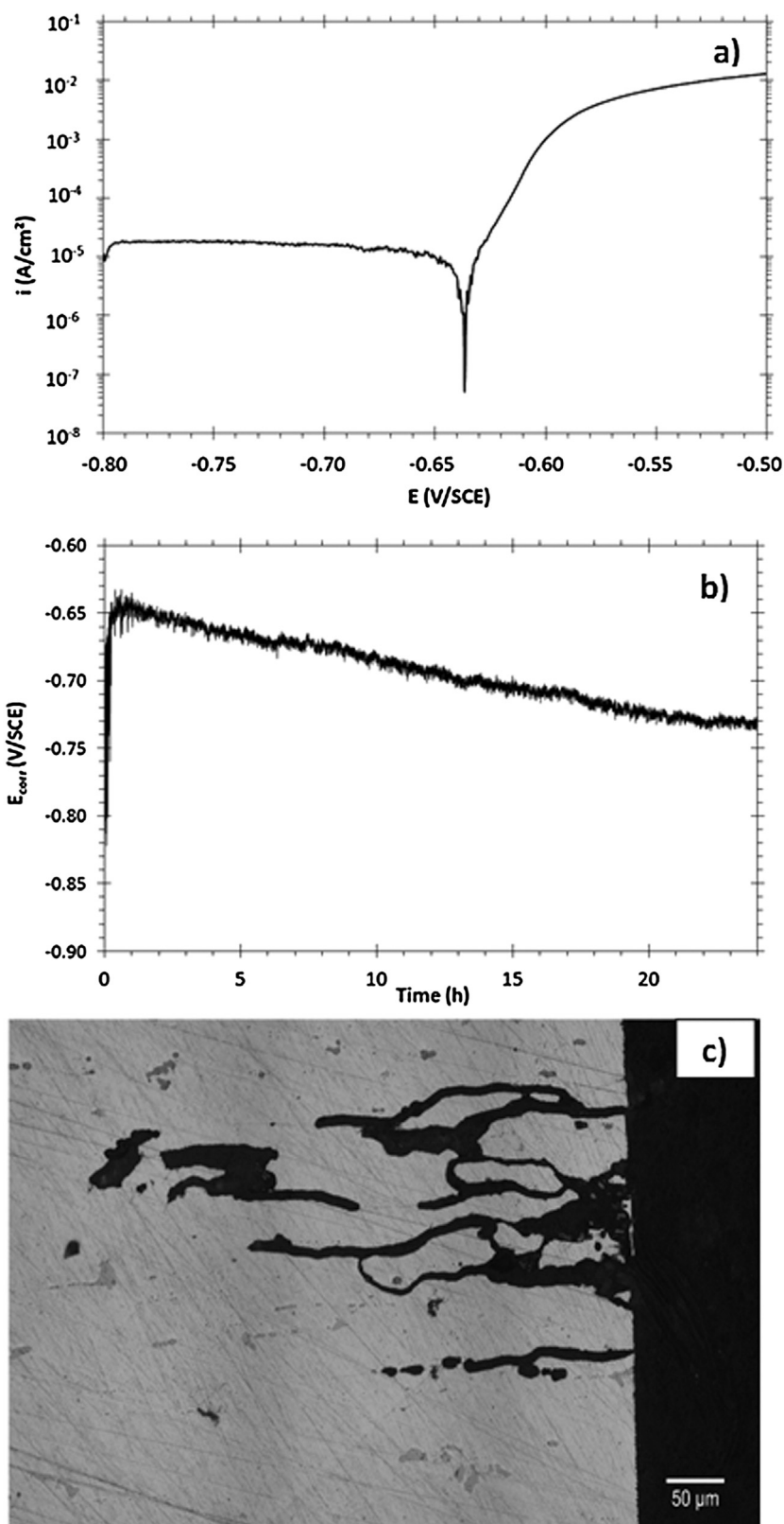
Fig. 1. a) Polarization curve of the AA2024 sample in a 1 M NaCl solution, b) E_{corr} versus the exposure time to 1 M NaCl solution, c) Optical micrograph of intergranular corrosion defects formed after a 24 h exposure at E_{corr} in a 1 M NaCl solution.
