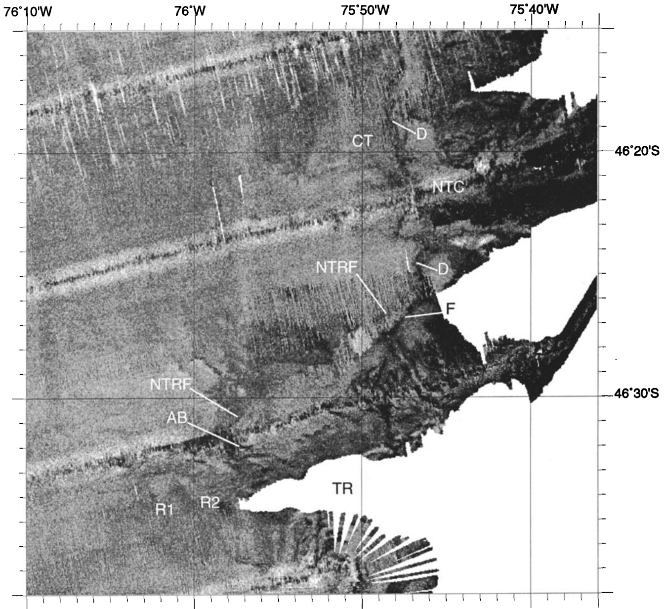
Figure 16. EM12 imagery of the Taitao Ridge subsegment. Note the low reflectivity of most of the area covered by the Taitao Ridge, including the scarp along the North Taitao Ridge fault. Acoustic basement of volcanic origin (AB); Chile trench (CT); decollement (D), fault (F); North Taitao canyon (NTC); North Taitao Ridge fault (NTRF); ridge 1 (R1); ridge 2 (R2); Taitao Ridge (TR). See text and Figure 13 for more details. Location is shown on Plate 1.
