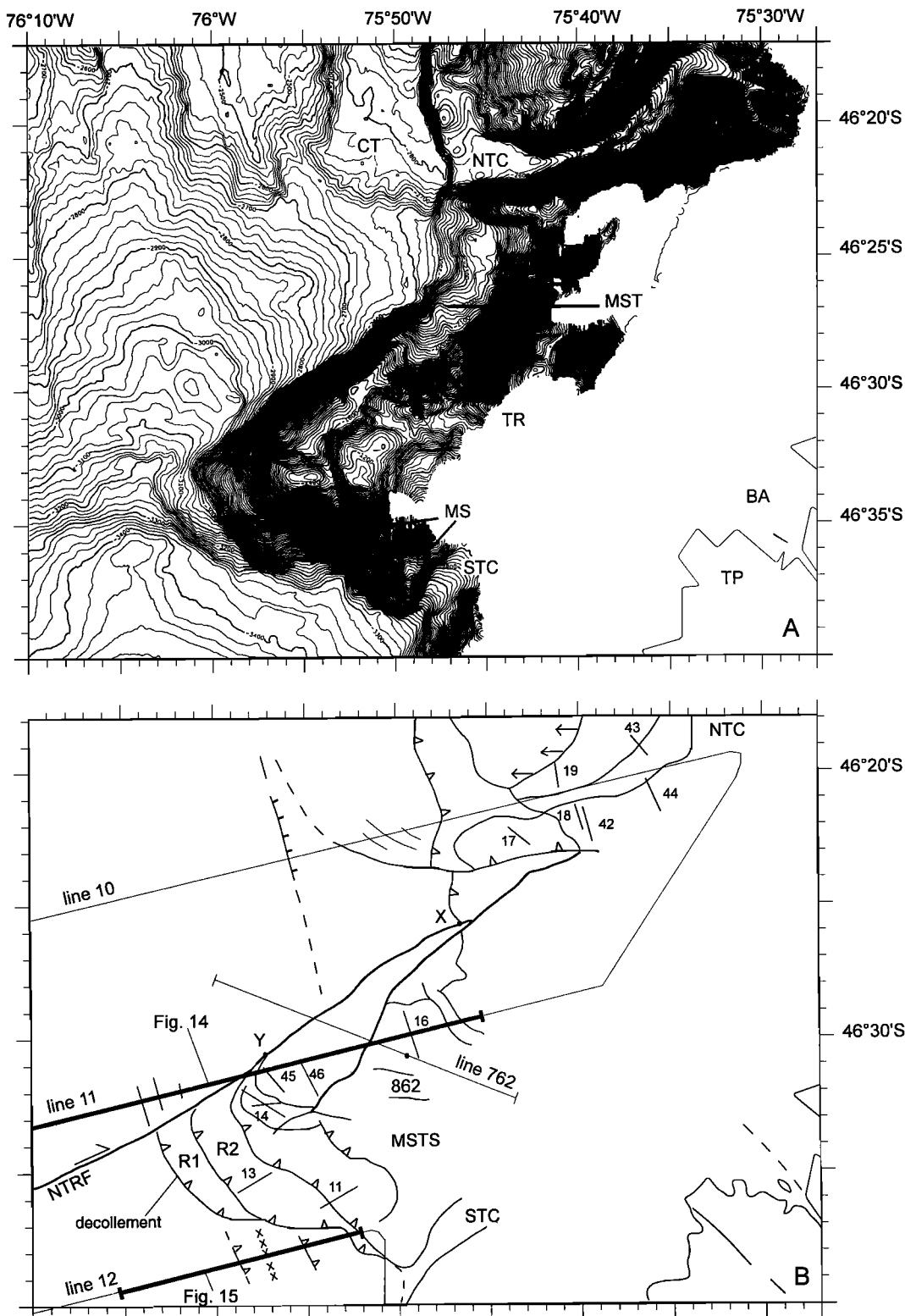
Figure 13. The Taitao Ridge subsegment along the synsubduction segment. (a) Bathymetric map (contours are every 20 m). (b) Structural sketch of the area shown in Figure 13a. Note that the structural sketch includes EM12 imagery data shown in Figure 16. Line with tick marks shows normal fault; line with open triangles shows thrust fault including the major decollement at the subduction front; solid dot marks the ODP Site 862. Locations of Figures 14 and 15 are shown. Bahia San Andres (BSA); Chile trench (CT); main scarp (MS); middle slope terrace (MST); main scarp thrust sheet (MSTS); North Taitao canyon (NTC); North Taitao Ridge fault (NTRF); ridge 1 (R1); ridge 2 (R2); South Taitao canyon (STC); Taitao peninsula (TP); Taitao ridge (TR). Dredge sites (11, 13, 14, 16, 17, 18, 19, 42, 43, 44, 45, 46, and the thick short lines in Figure 13a). Letters X and Y refer to descriptions in the text. See text for more details. Location is shown on Plate 1.
