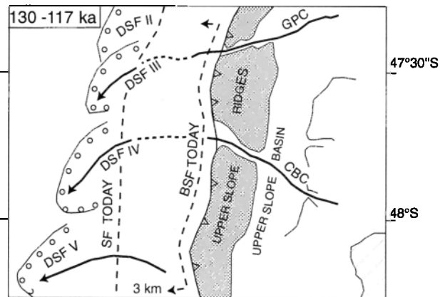
Figure 26. Reconstruction of the Chile continental margin and trench along the postsubduction segment at 130-117 ka. At that time, the decollement was located along the toe of the Upper Slope ridges. The deep-sea fans (DSF) III and IV connected with the outflow of the Golfo de Penas and Cabo Bynoe canyons, respectively. The dashed lines show the present location of the subduction front (SF) and the back stop front (BSF) resulting from 3 km of convergence between the Antarctic and South America plate during the past 130-117 kyr. Cabo Bynoe canyon (CBC); Golfo de Penas canyon (GPC). See text for more detail.
