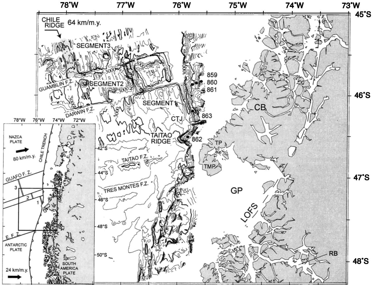
Figure 1. Bathymetric map of the region surveyed during the CTJ cruise of the R/V L'Atalante in the Chile triple junction area, between 45°S and 48°S. The main seafloor morphological features include the Chile ridge axes and fracture zones, the Chile trench, and the Andean continental margin. Location map is shown in the inset. Numbers 859 to 863 refer to the ODP sites drilled during ODP Leg 141. Chile triple junction (CTJ); Chiloe block (CB); Esmeralda fracture zone (EFZ); Golfo de Penas (GP); Liquine-Ofqui fault system (LOFS); Rio Baker (RB); Tres Montes peninsula (TMP); Taitao peninsula (TP).
