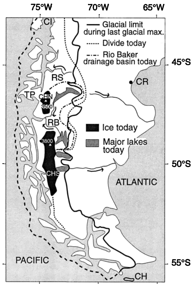
Figure 4. Limits of the last glacial maximum and distribution of existing ice field. Campo de Hielo Norte (CHN); Campo de Hielo Sur (CHS); Cabo de Horn (CH); Chiloe Island (CI); Comodoro Rivadavia (CR); Rio Baker (RB); Rio Simpson (RS); Taitao peninsula (TP). Note that the development of the ice cap during the Last Glacial Maximum prevents drainage to the Pacific as the Rio Baker acts today.
