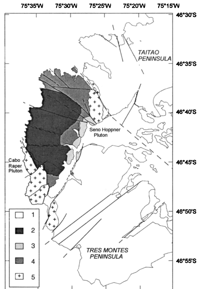
Figure 3. Simplified geologic map of the Taitao peninsula after Mpodozis et al. [1985], Forsythe et al. [1986], and Bourgeois et al. [1996]. Units are as follow: 1, pre-Jurassic metamorphic basement; 2, Bahia Barrientos ophiolite; 3, Chile margin unit; 4, main volcanic unit; 5, Pliocene plutons.
