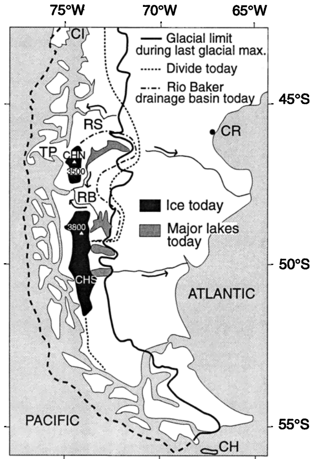
Figure 4. Limits of the last glacial maximum and distribution of existing ice field. Campo de Hielo Norte (CHN); Campo de Hielo Sur (CHS); Cabo de Horn (CH); Chiloe Island (CI); Comodoro Rivadavia (CR); Rio Baker (RB); Rio Simpson (RS); Taitao peninsula (TP). Note that the development of the ice cap during the Last Glacial Maximum prevents drainage to the Pacific as the Rio Baker acts today.
