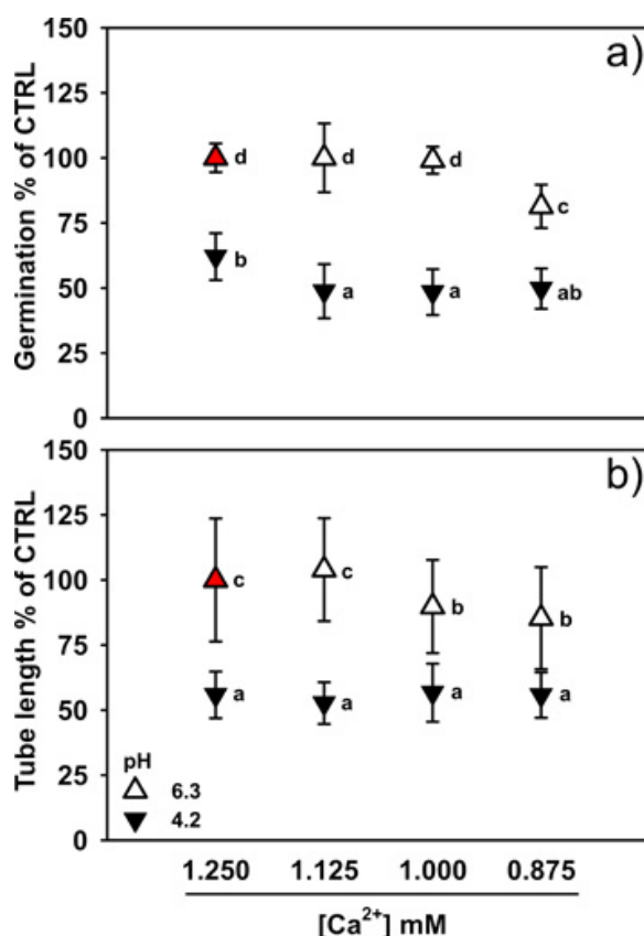
Fig. 4. Effect of \text{Ca}^{2+} and/or pH decrease on C. avellana pollen performance. Pollen germination percentage (a) and tube length (b) after 3 h of incubation in BK (CTRL: red triangle), BK with a decreased \text{Ca}^{2+} concentration, pH or both. Values are reported as means \pm 1 st. dev. [ n = 450 for a); n \geq 50 for b)]. Statistically different groups are marked with different letters (Two-way Anova, Fisher's LSD test) (For interpretation of the references to colour in this figure legend, the reader is referred to the web version of this article).
