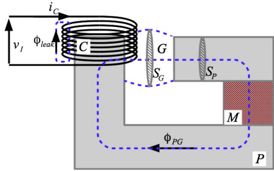
(a) Schematic
