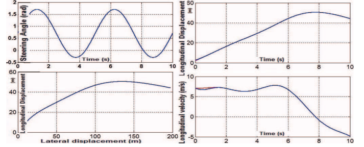
Figure 3. Vehicle behavior for a sinusoidal steering
