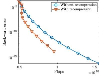
(B) Flops–accuracy tradeoff. Each point corresponds to a different \epsilon threshold.
