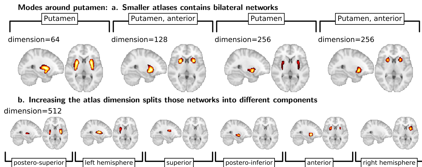
Figure A8: Interpretation of higher-dimensional modes of DiFuMo: The putamen segmentation is refined as dimension of DiFuMos increases. A single mode contain the left and right putamen in lower dimension (a), when higher order atlases holds separate components for them. Larger atlases model the detailed organization within the sub-structures, which may be crucial in discriminative tasks.
