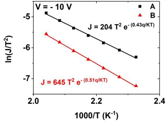
Figure 5 : Linear fit (straight lines) of experimental data points (scatters) for SBDs A and B. The current density J is expressed in A.m^{-2} .
