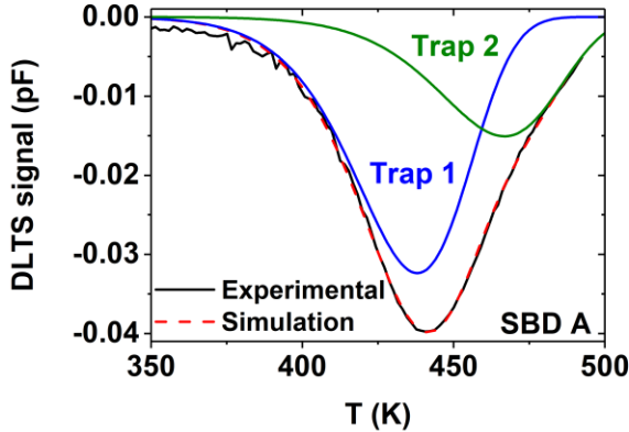
Figure 13 : Simulation using equations 2-4 of the experimental DLTS spectrum of diode A shown in Fig. 6.
