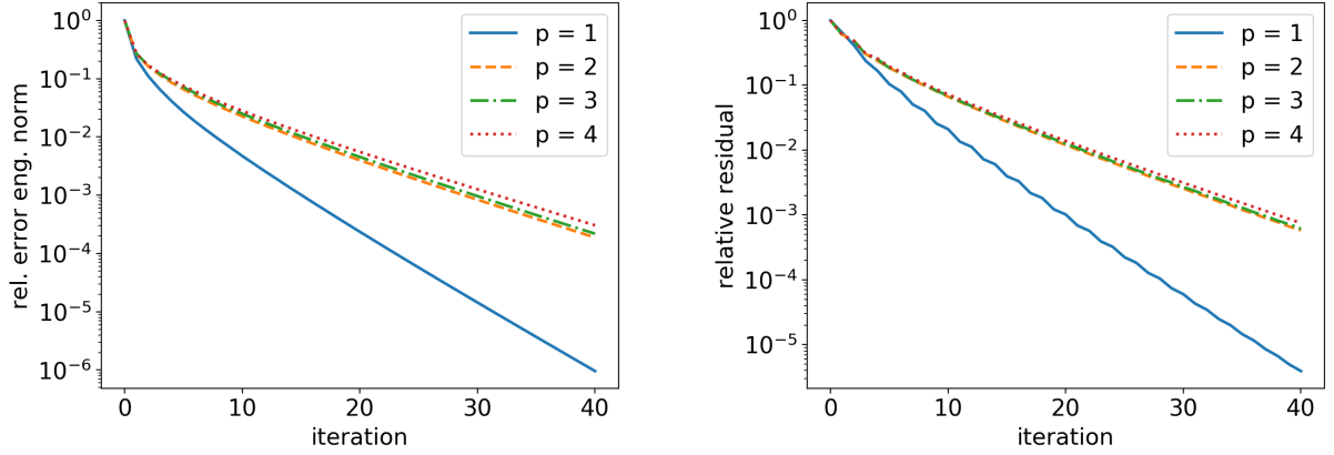
Figure 6: Cube case: decay of the relative algebraic error (left) and the relative residual (right) for the hierarchy with p_j = 1, j \in \{1, \dots, J-1\}, J = 4 . The solver of Definition 4.1 is stopped at iteration i = 40 . nDoFs: 5 501 for p = 1 , 41 337 for p = 2 , 136 693 for p = 3 , 320 753 for p = 4 .
