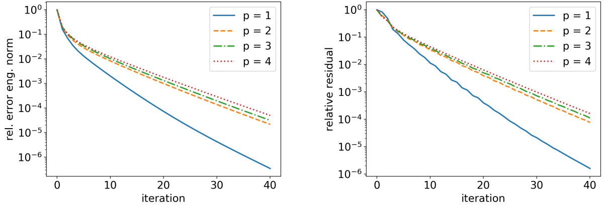
Figure 7: Nested cubes case: decay of the relative algebraic error (left) and the relative residual (right) for the hierarchy with p_j = 1, j \in \{1, \dots, J-1\}, J = 4 . The solver of Definition 4.1 is stopped at iteration i = 40 . nDoFs: 7 281 for p = 1 , 55 649 for p = 2 , 185 041 for p = 3 , 435 393 for p = 4 .
