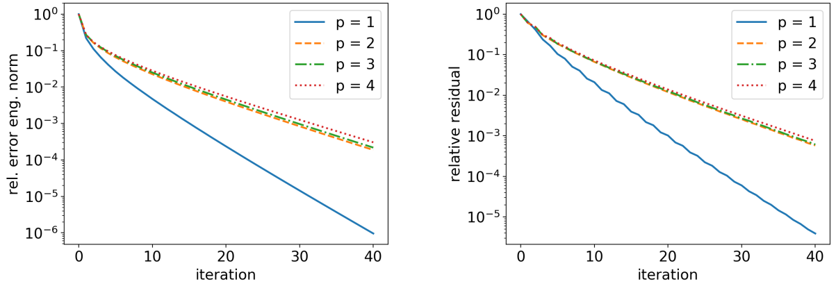
Figure 6: Cube case: decay of the relative algebraic error (left) and the relative residual (right) for the hierarchy with p_j = 1, j \in \{1, \dots, J-1\}, J = 4 . The solver of Definition 4.1 is stopped at iteration i = 40 . nDoFs: 5 501 for p = 1 , 41 337 for p = 2 , 136 693 for p = 3 , 320 753 for p = 4 .
