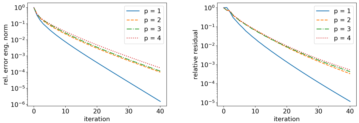
Figure 8: Checkers cubes: decay of the relative algebraic error (left) and the relative residual (right) for the hierarchy with p_j = 1, j \in \{1, \dots, J-1\}, J = 4 . The solver of Definition 4.1 is stopped at iteration i = 40 . nDoFs: 5 425 for p = 1 , 40 033 for p = 2 , 131 473 for p = 3 , 307 393 for p = 4 .
