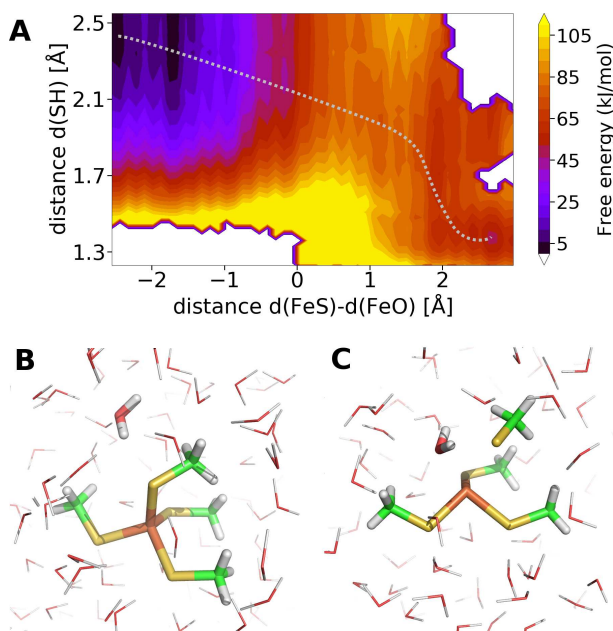
Figure 2: Hydrolysis of \text{Fe}(\text{SCH}_3)_4^- (reaction A in Fig. 1) in explicit solvent. (A) Two-dimensional free energy profile for the reaction in aqueous solution obtained with a hybrid QM/MM potential. Gray dashed line shows the approximate minimum free energy pathway. Snapshots of the (B) reactant and (C) transition states show the reactive atoms in sticks with Fe in orange, S in yellow, O in red and C in green.
