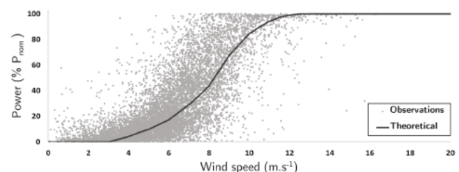
Figure 1: Production and wind speed relationship
