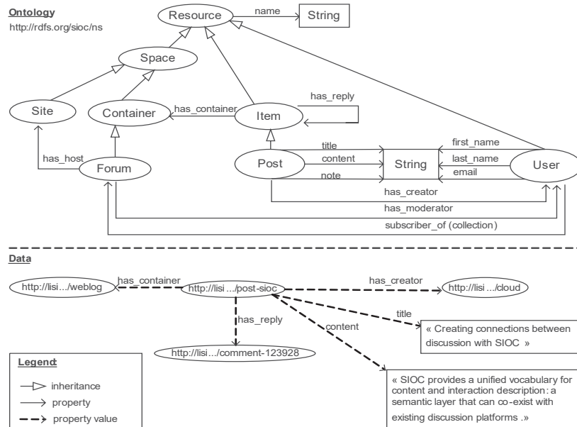
Fig. 1. A graphical representation of a toy ontology
