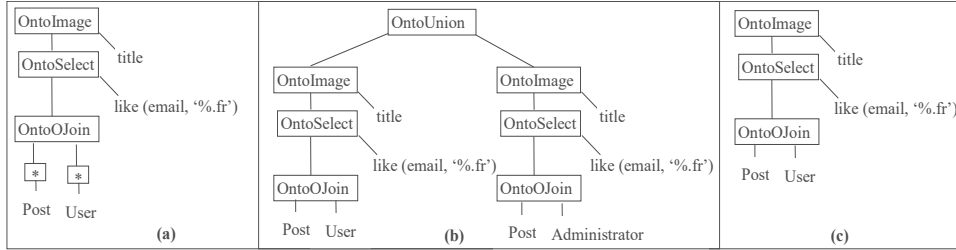
Fig. 2. Example of an optimization based on a partial evaluation technique
