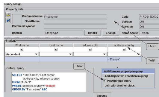
Fig. 4. OntoQBE: a graphical editor for OntoQL queries similar to QBE
