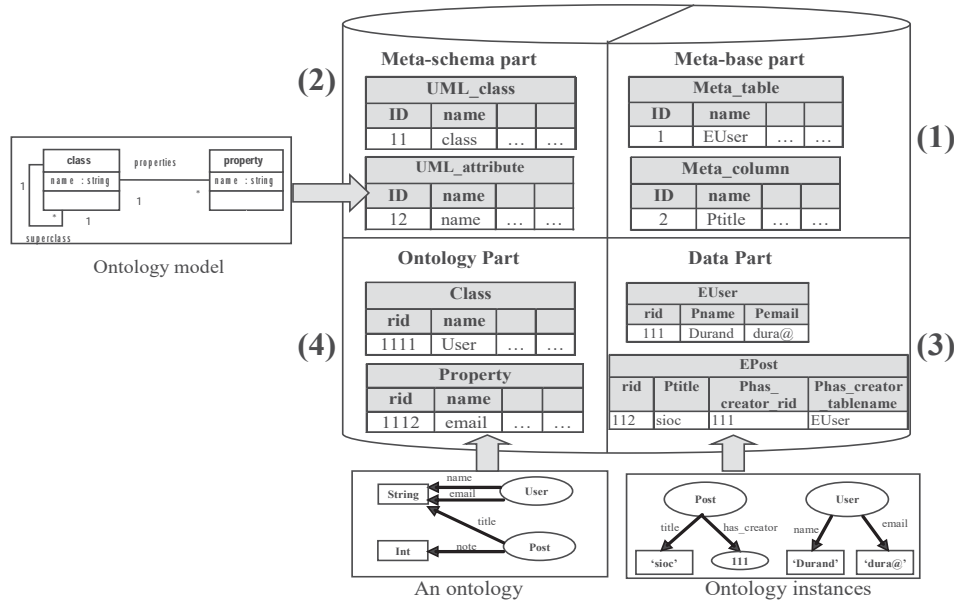
Fig. 3. The OntoDB 4-parts architecture
