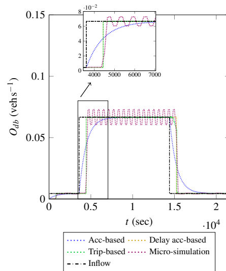
(f) Outflow vs. time for buses in dedicated bus lanes.
