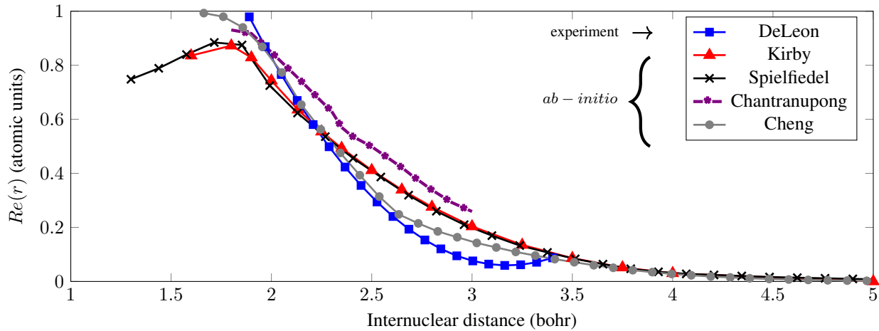
Figure 1: Electronic transition moment function ( Re(r) ) taken from Kirby and Cooper, 14 Spielfiedel et al, 15 Chantranupong et al, 16 Cheng et al 17 and DeLeon. 18,19
