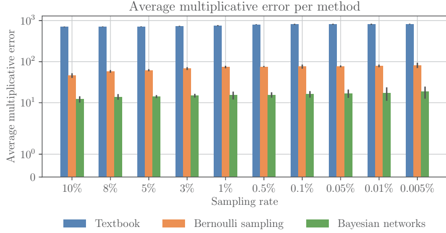
Fig. 4. Average errors
