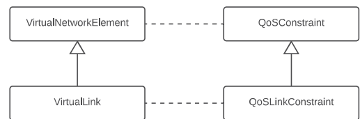
Fig. 7. Specialization of QoS model
