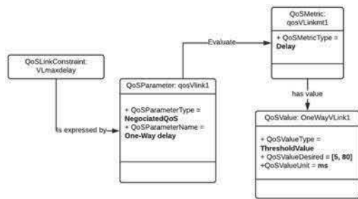
Fig. 9. QoS model instantiation to the virtual link constraints
