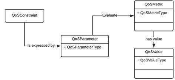
Fig. 3. QoSConstraint model: QoSMetric representation
