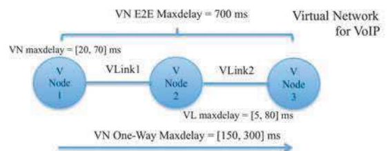
Fig. 8. Example of VN QoS constraints for VoIP
