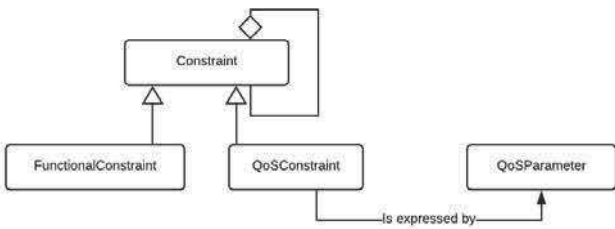
Fig. 2. Constraint Model
