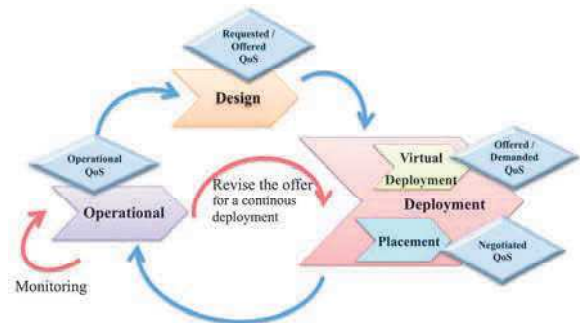
Fig. 6. QoS and service lifecycle: towards a continuous deployment
