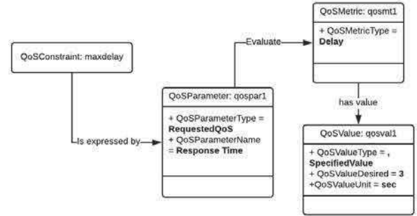
Fig. 4. Example of instantiation of QoSConstraint Model
