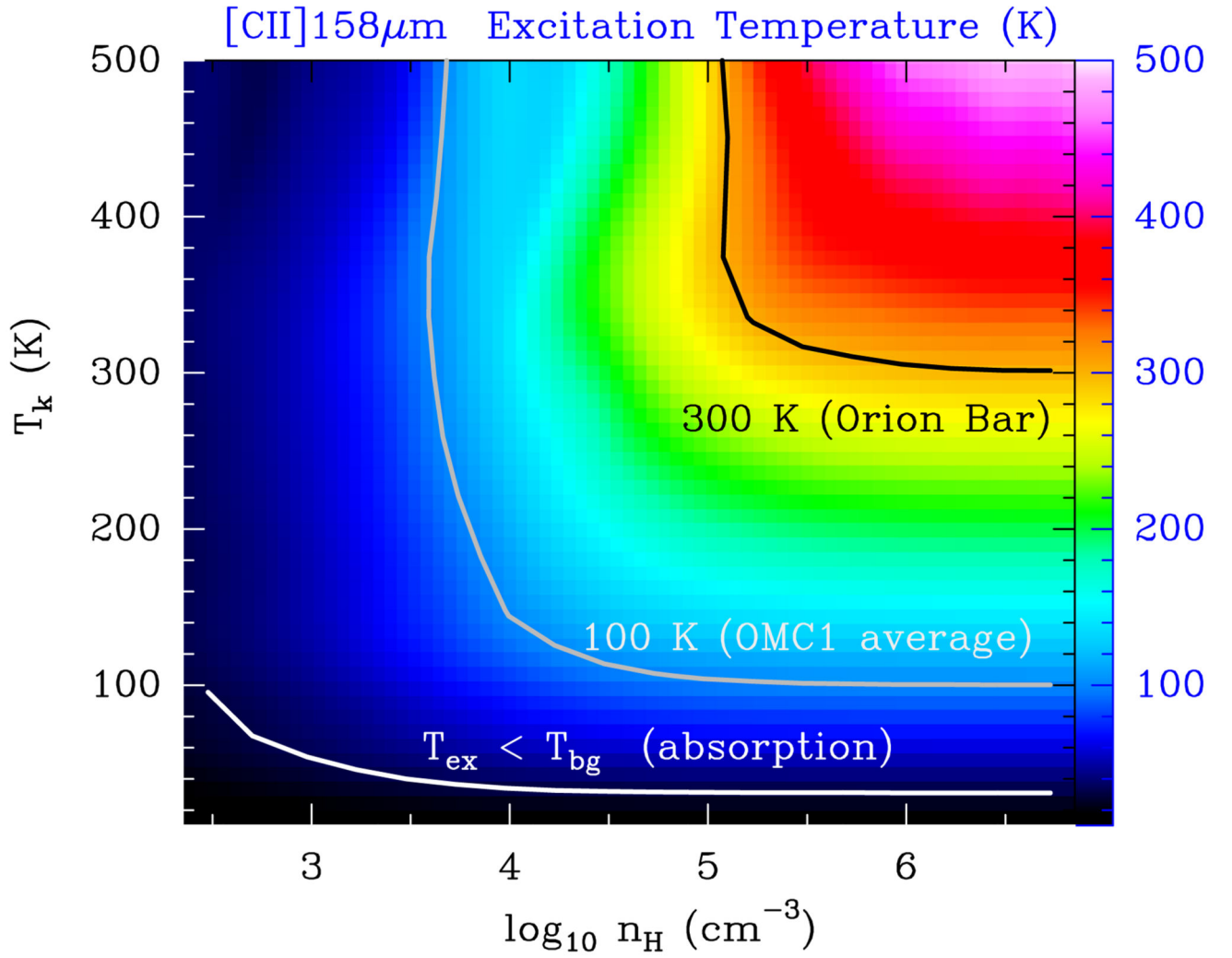
Figure 10. Synthetic excitation temperatures for the [\text{C II}] 158 \mu\text{m} transition obtained from a grid of nonlocal non-LTE models (see text).
