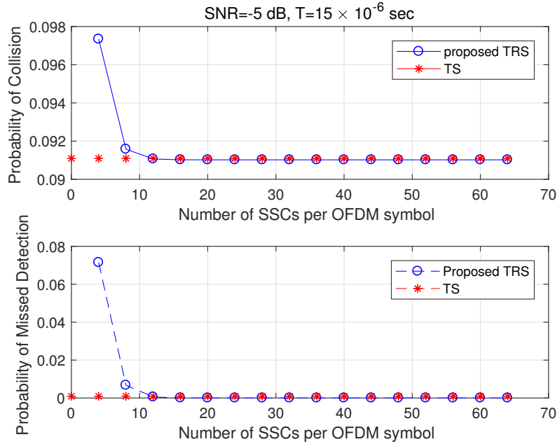
(a) P_c and P_{md} Vs. Number of SSCs
