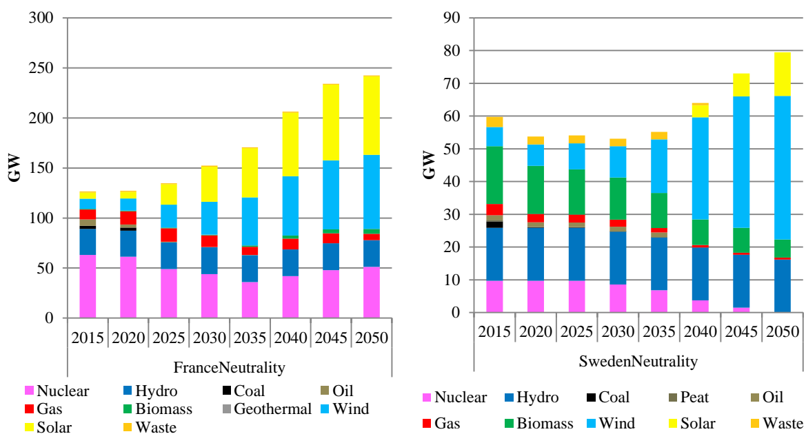
Figure 4 Power plant capacities
