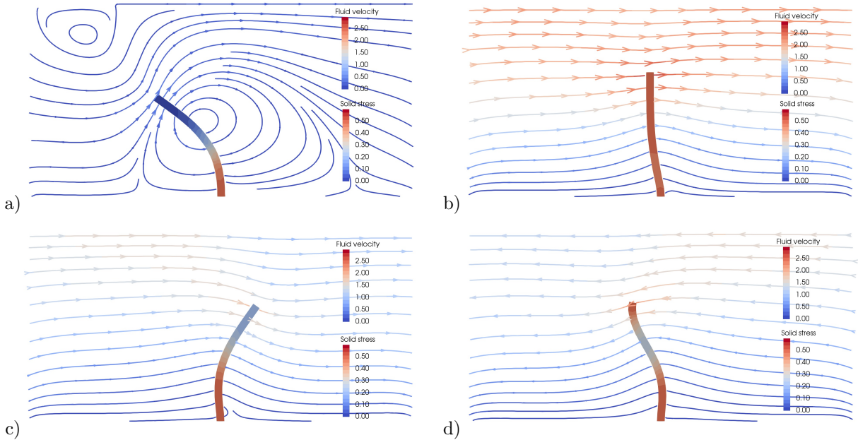
Figure 6: One cilium beating in a viscous fluid of viscosity \mu_f = 0.01\text{pN} \cdot \mu\text{m} \cdot \text{s} at different times: a) t = 0.091s , b) t = 0.110s , c) t = 0.120s and d) t = 0.166s . The activity scenario of the structure is given by (7).
