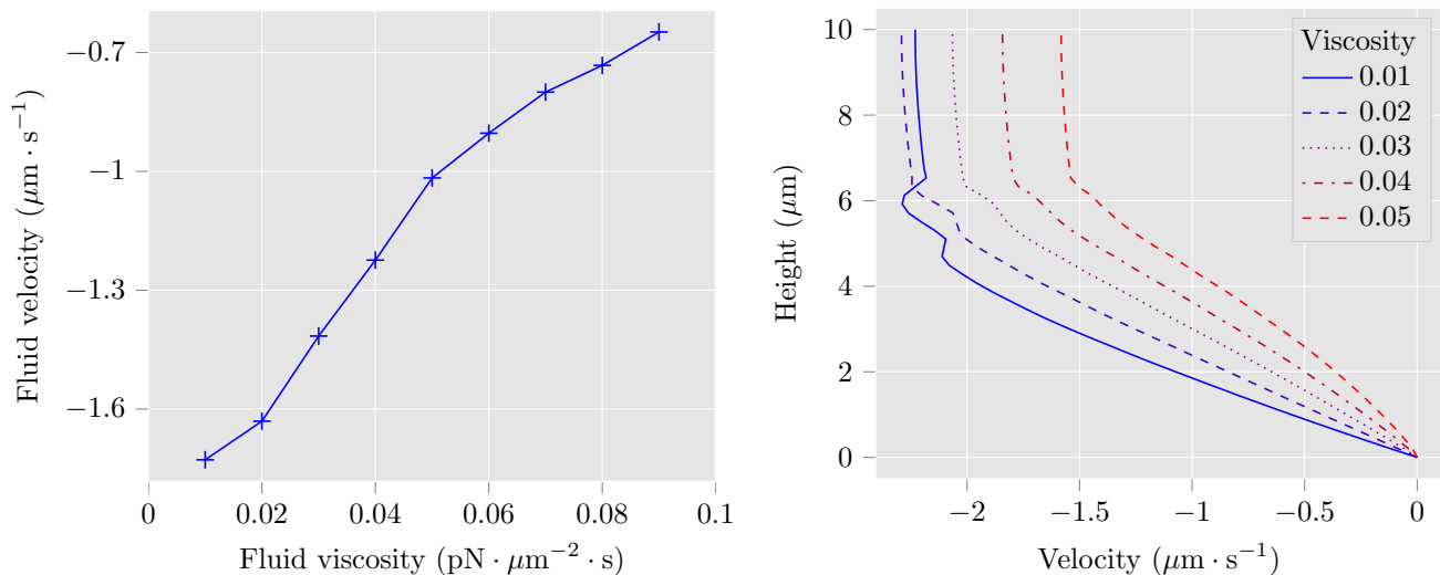
Figure 11: a) Time average of the horizontal fluid velocity in function of the viscosity of the fluid and b) horizontal velocity of the fluid as a function of the height for different values of the viscosity.
