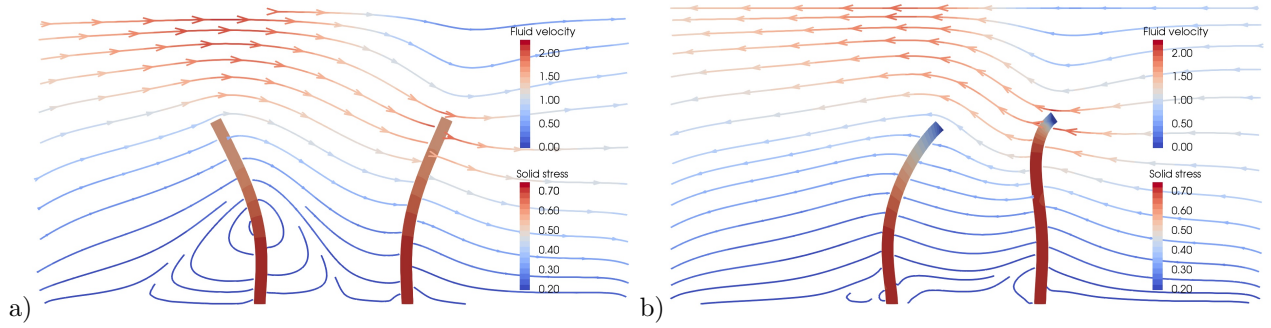
Figure 12: Two cilia beating in a viscous fluid with \mu_f = 0.01 \text{pN} \cdot \mu\text{m}^{-2} \cdot \text{s} at a) t = 0.788\text{s} and b) t = 0.83\text{s} . The cilia are anchored at x_{c_1} = 7.5\mu\text{m} and x_{c_2} = 12.5\mu\text{m} . The phase shift between the two cilia is \delta\phi = 0.075\text{s} .
