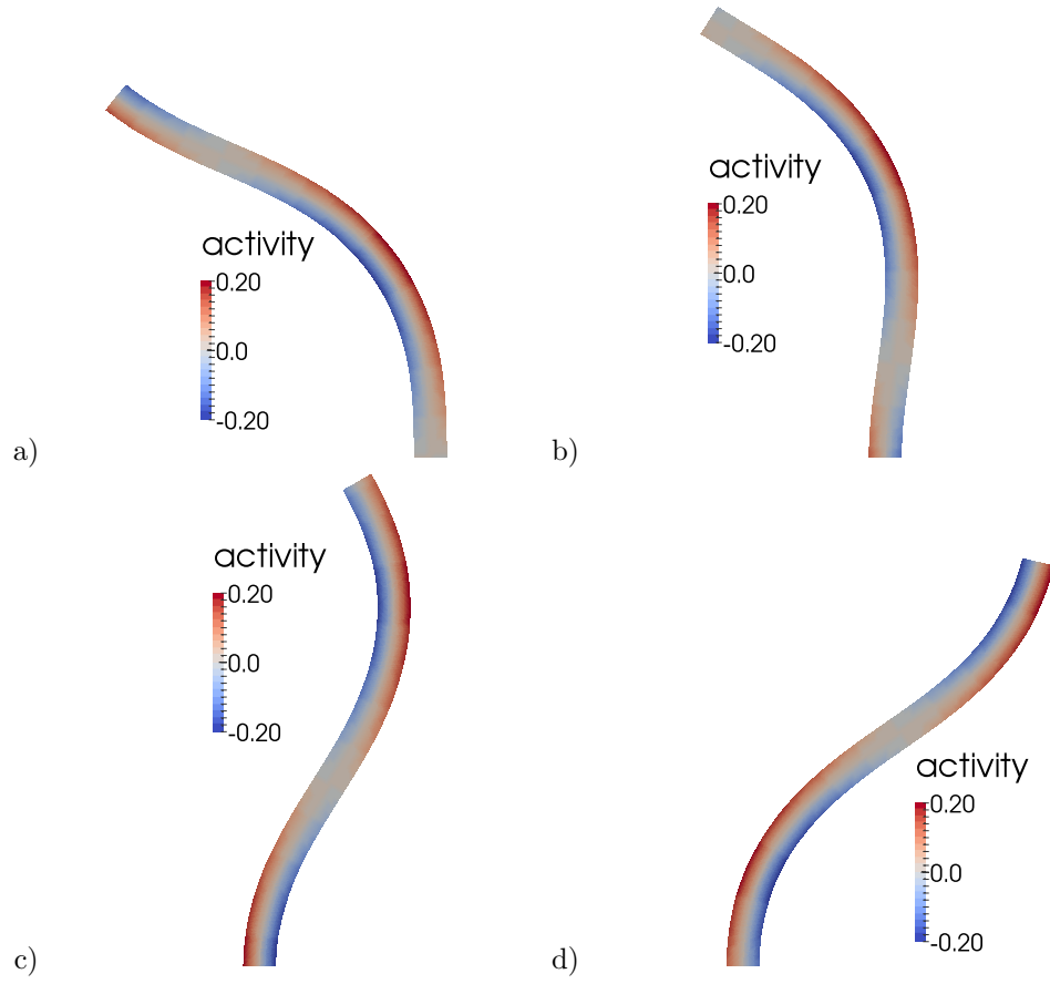
Figure 2: Deformation of an elongated structure subjected to the internal activity defined by (6) at different times: a) t = 0s , b) t = 0.012s , c) t = 0.025s and d) t = 0.037s . The activity scenario \Sigma_a is represented with the set of parameters be given in Table 2.
