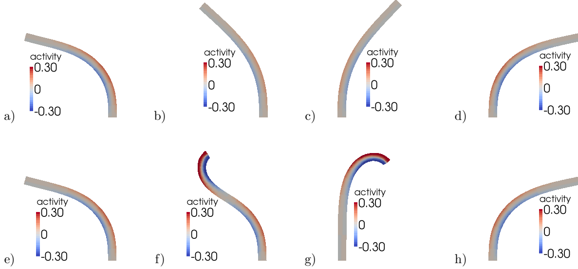
Figure 3: Elongated structure subjected to the internal activity defined by (7) inducing cilia-like deformations at different time: a) t = 0\text{s} , b) t = 0.015\text{s} , c) t = 0.035\text{s} , d) t = 0.050\text{s} , h) t = 0.050\text{s} , g) t = 0.065\text{s} , f) t = 0.085\text{s} and e) t = 0.1\text{s} . The activity scenario \Sigma_a is represented with the set of parameters be given in Table 3.
