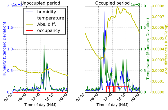
Fig. 7. Absolute difference of Humidity and Temperature Sigma versus occupancy.
