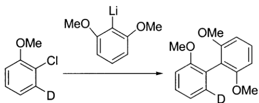
Scheme 4. Ipso substitution reaction on deuterated substrate.
