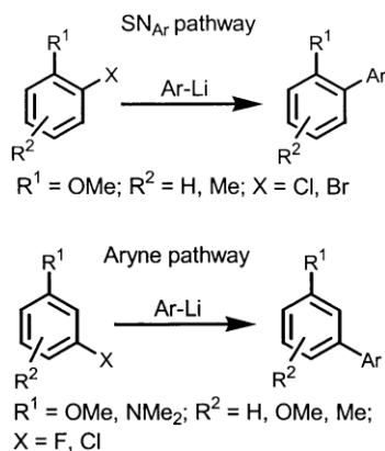
Scheme 5. Summary of the substrate substitution reaction pathways.
