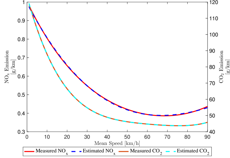
Figure 2: Reference and estimated emission factor of \text{NO}_x and \text{CO}_2 for varying mean speed.
