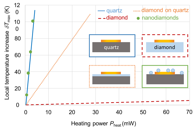
FIG. 3. Numerical simulations of the maximum local heating \delta T_{\text{max}} at the sample surface induced by a two-dimensional 10 \times 10 \mu\text{m}^2 heater for increasing heat powers P_{\text{heat}} ; four configurations are considered: the hot plate located either on a diamond substrate (red dash line), on a quartz substrate (blue solid line), on a 100-nm thick diamond membrane bonded on a quartz substrate (orange dotted line), or on a quartz substrate with diamond nanostructures dispersed on the surface (green dots); in this latter architecture, temperature increase is the one reached within the nanostructures whose dimensions are in the range of few tens of nanometers; the insets show schematics of the four configurations; the temperature increase per heating power reaches \approx 4 \text{ K/mW} in the heterostructure geometry; it is almost two orders of magnitude higher than the one predicted on bulk diamonds and is solely \approx 6 or 7 times smaller than the one expected on the quartz geometry.
